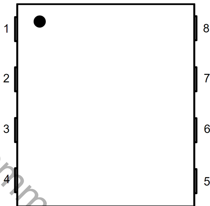
Figure 6.2. 8-Pin DFN, Top View
