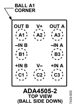
Figure 4. 8-Ball WLCSP (CB-8-2)
