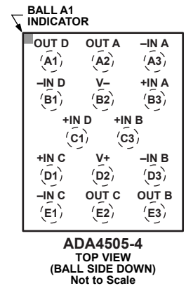
Figure 6. 14-Ball WLCSP (CB-14-1)
