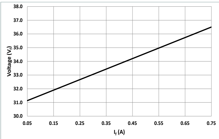
Forward Current vs. Forward Voltage @ 85°C
