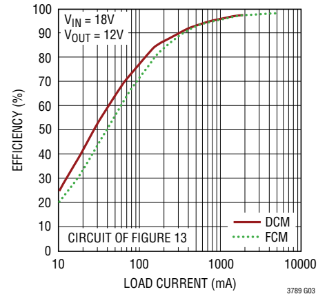
Efficiency vs Output Current (Buck Region)
