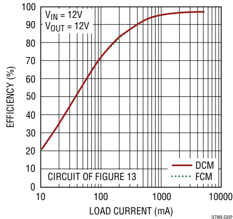
Efficiency vs Output Current (Buck-Boost Region)
