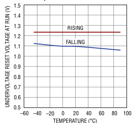
RUN Pin Threshold vs Temperature
