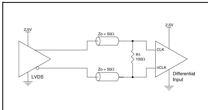
Figure 3C. CLK/nCLK Input Driven by a 2.5V LVDS Driver
