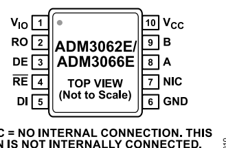
Figure 12. ADM3062E/ADM3066E 10-Lead MSOP Pin Configuration
