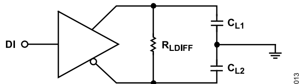
Figure 40. Driver Propagation Delay
