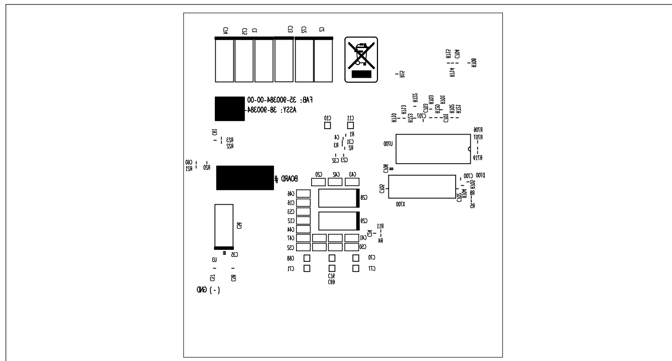
Bottom Silkscreen
