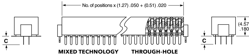
MIXED TECHNOLOGY THROUGH-HOLE
