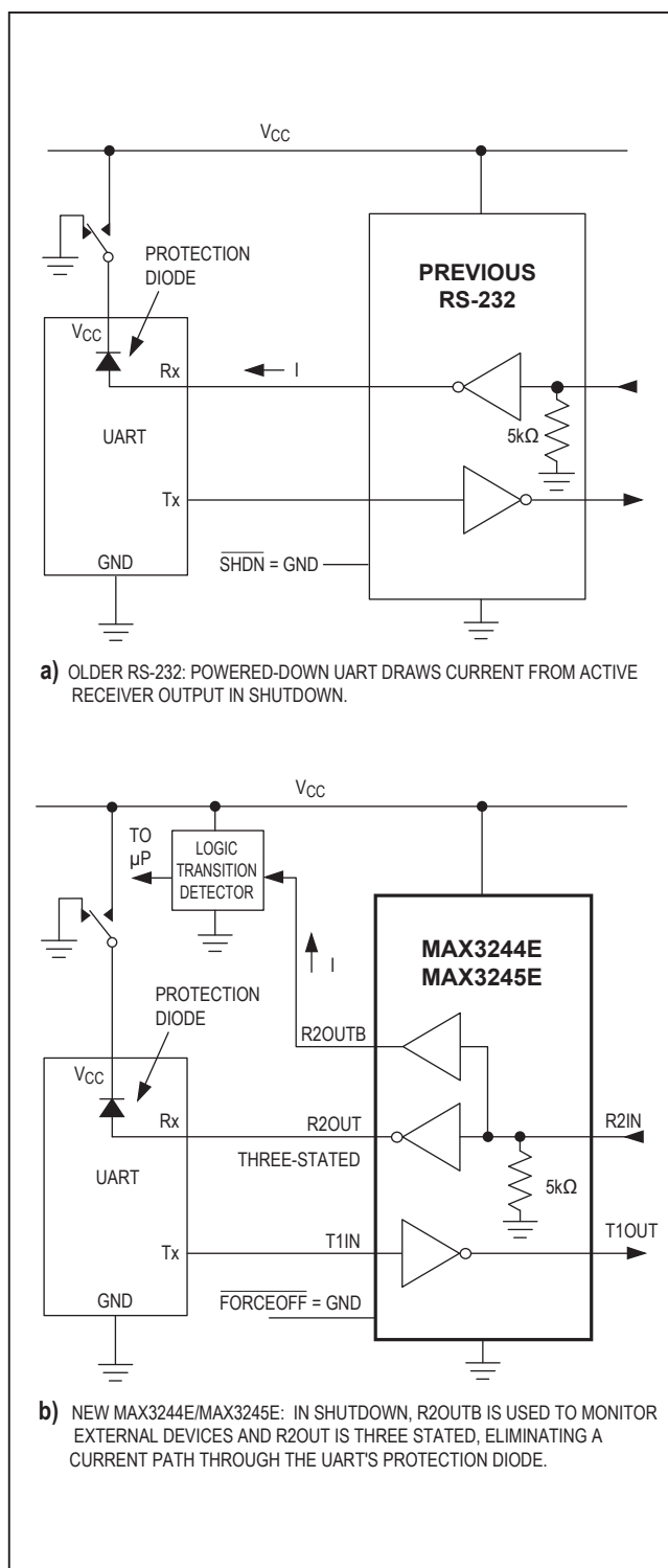
Figure 2. The MAX3244E/MAX3245E detect RS-232 activity when the UART and interface are shut down.
