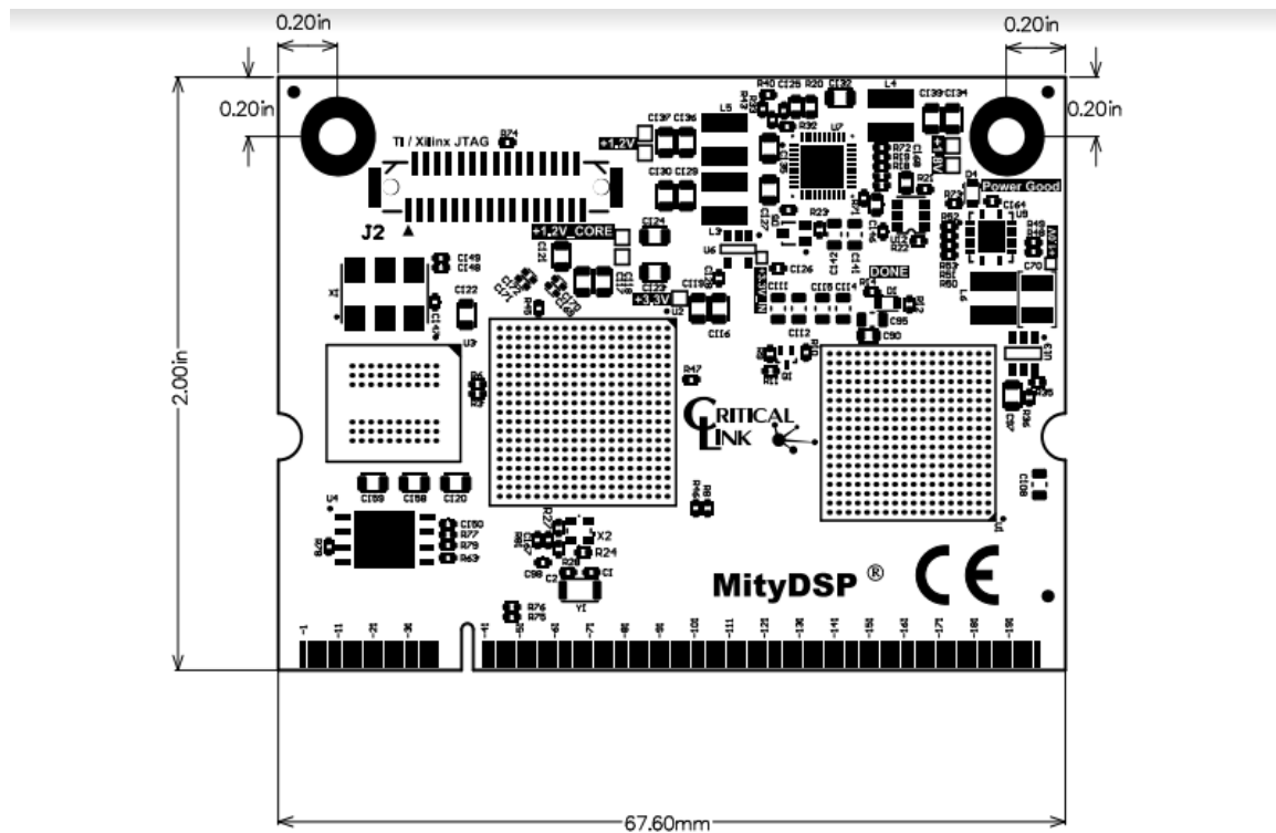
Figure 2 MityDSP-L138F-A7 Mechanical Outline
