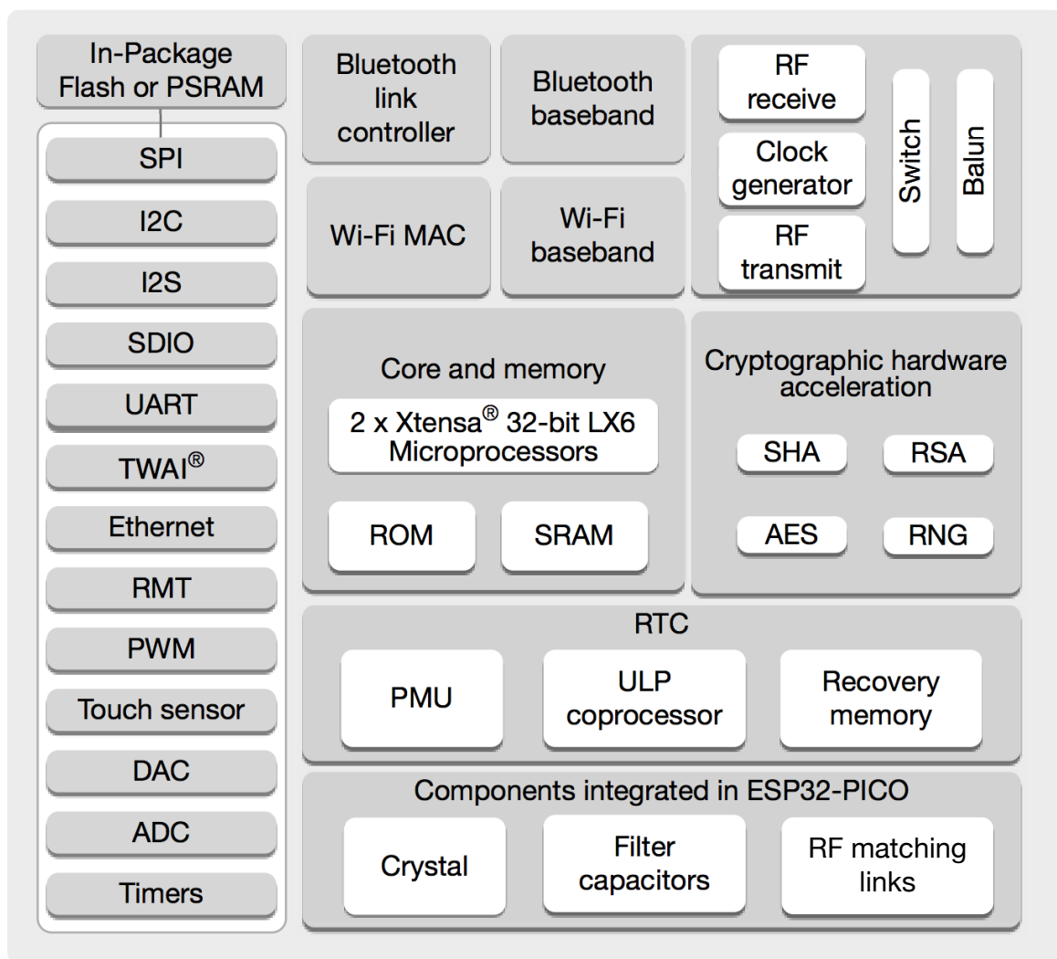
Figure 1: ESP32-PICO Functional Block Diagram
