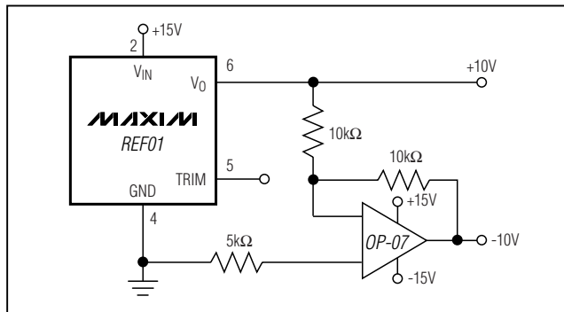
Figure 3. ±10V Reference
