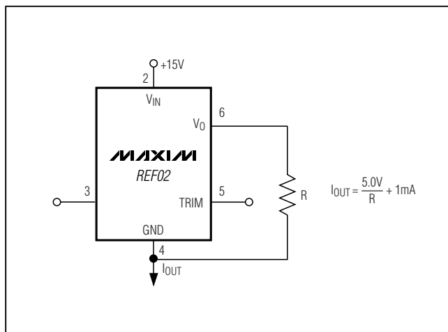
Figure 4. Current Source
