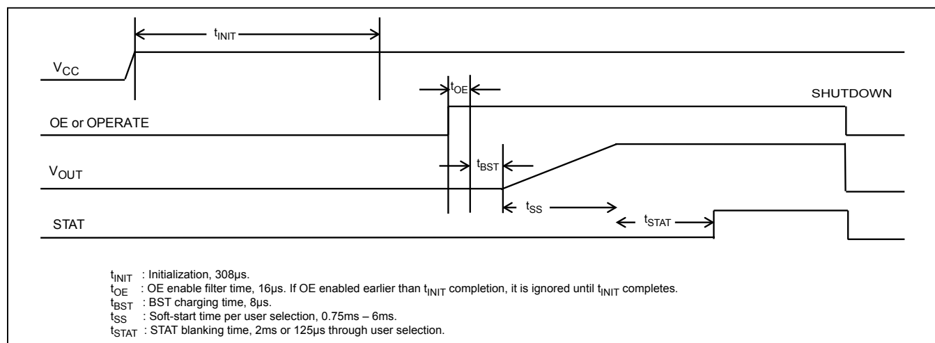
Figure 1. Startup Timing
