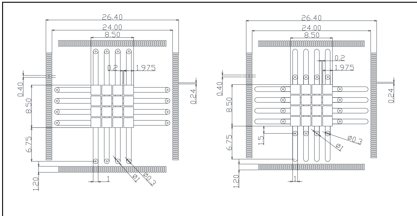
Figure 8-4: Optional Land Pattern
