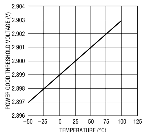
Power Good Threshold Voltage vs Temperature ( 3V_{\text{OUT}} )
