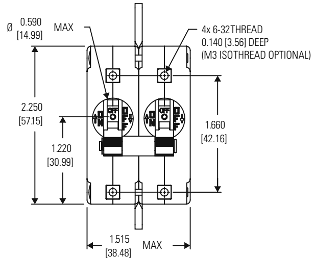
PANEL MOUNT CUTOUT - 2 POLE, 2 HANDLE
