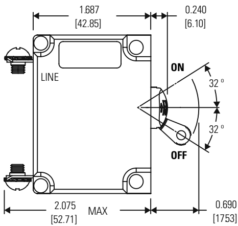
TWO POLE, 2 HANDLE
