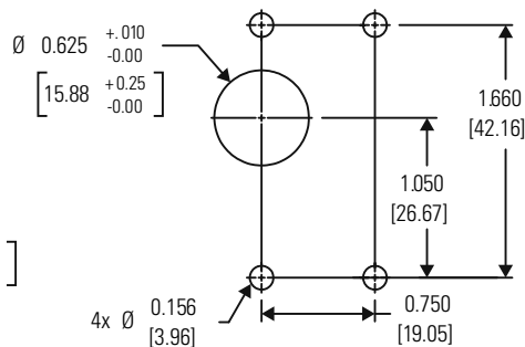
PANEL MOUNT CUTOUT - 2 POLE, 1 HANDLE
