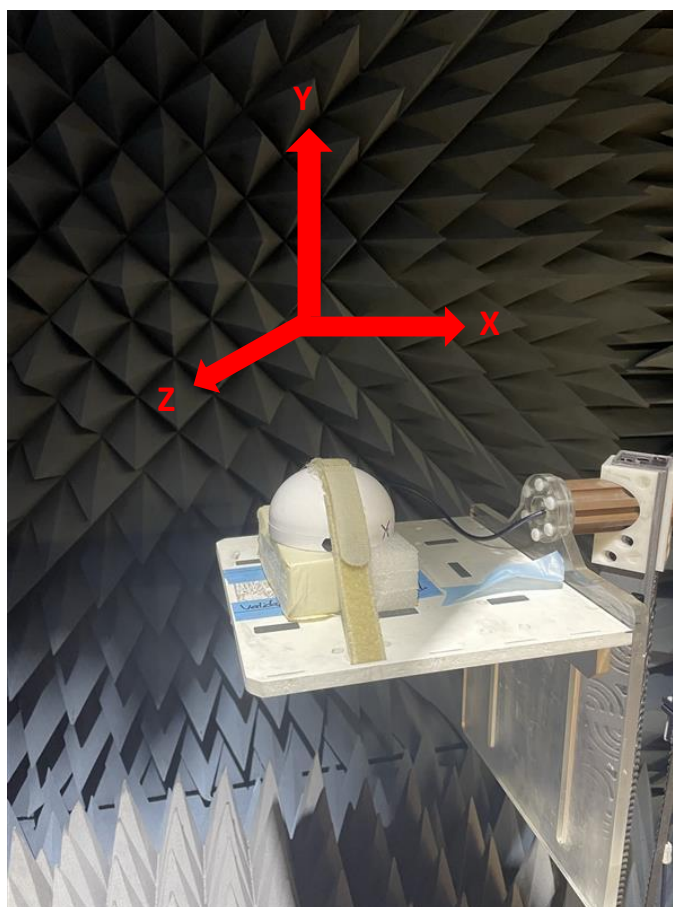
Chamber Test-Setup
