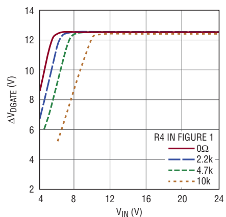
\Delta V_{DGATE} vs V_{IN} in Figure 1
