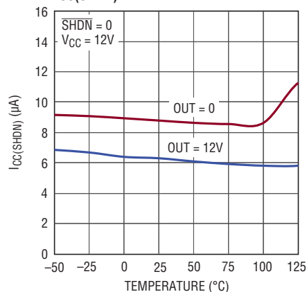
I_{CC(SHDN)} vs Temperature
