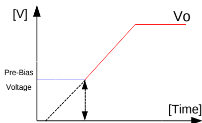
Figure 16: Pre-Bias startup
