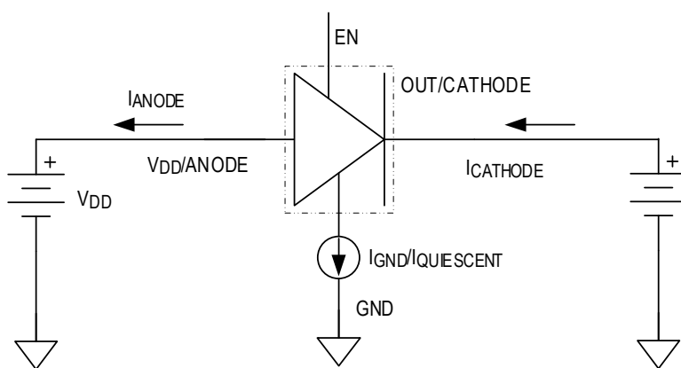
REVERSE-BIASED CONDITION
