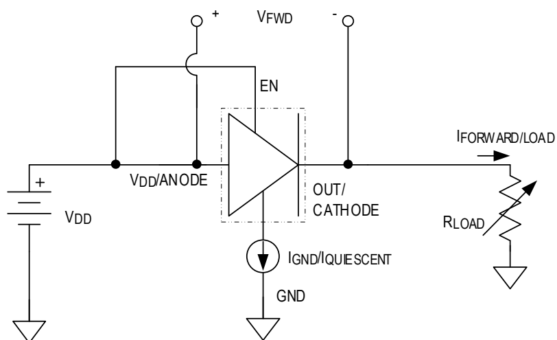
FORWARD-BIASED CONDITION
