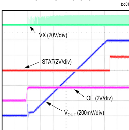
STARTUP RESPONSE
