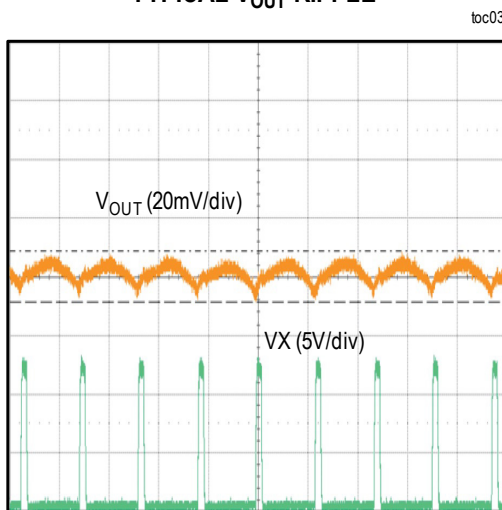
TYPICAL V_{OUT} RIPPLE
