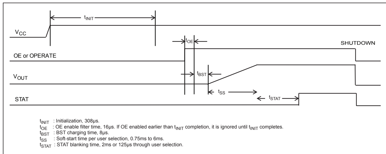
Figure 1. Startup Timing
