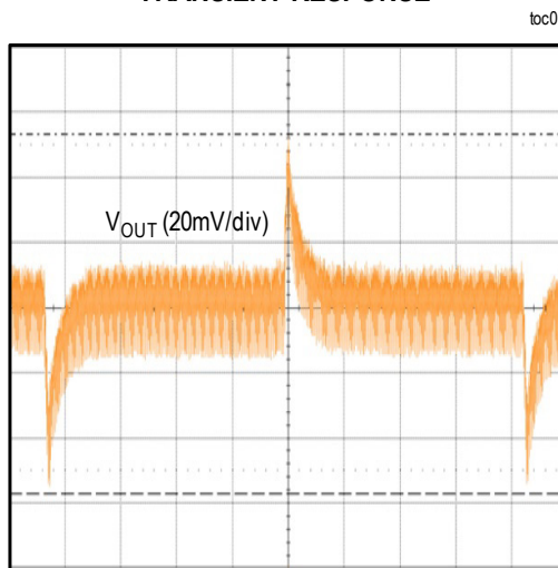
TRANSIENT RESPONSE
