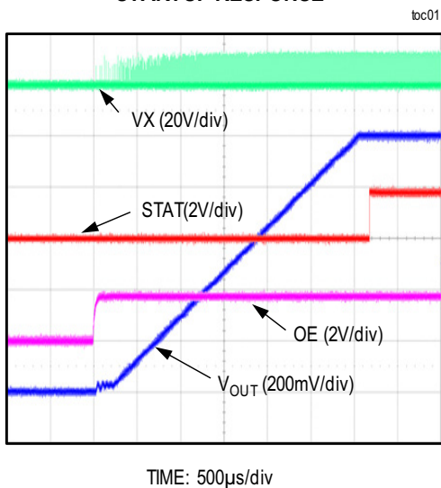
STARTUP RESPONSE
