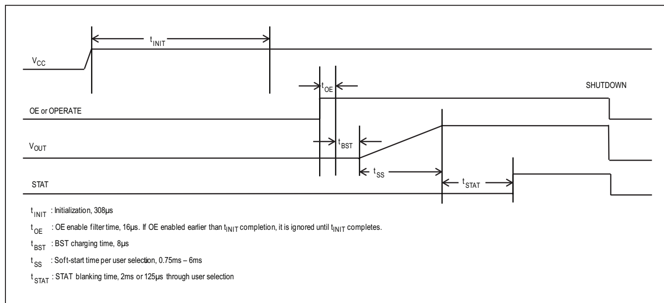
Figure 1. Startup Timing
