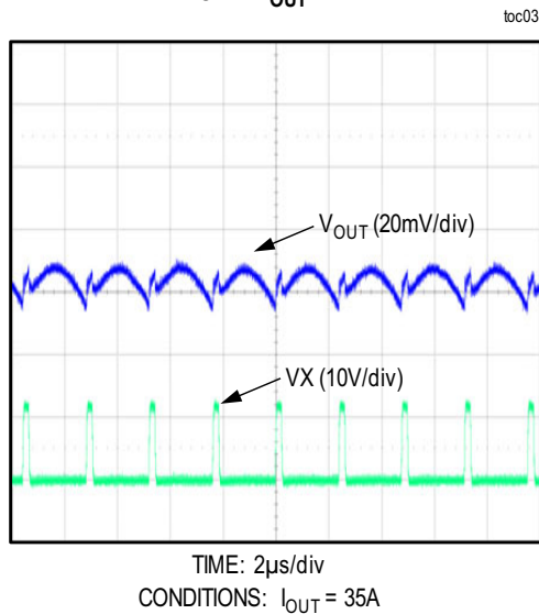
TYPICAL V_{OUT} RIPPLE
