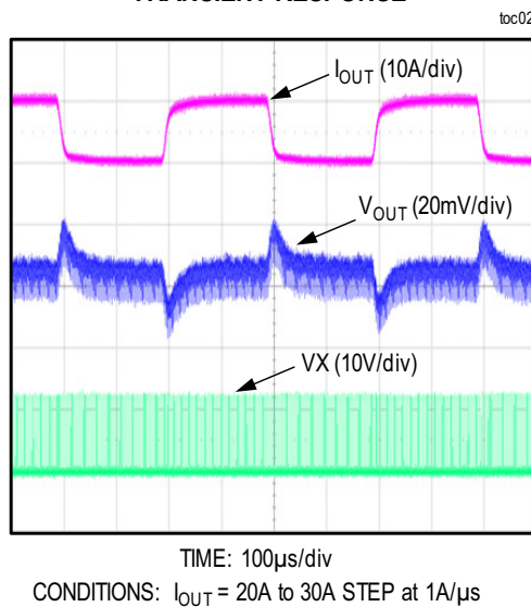
TRANSIENT RESPONSE
