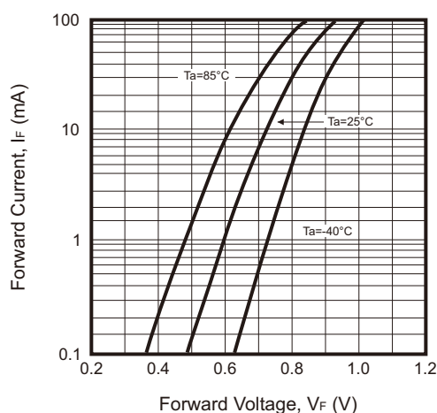
Fig.1 - Forward Voltage
