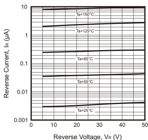
Fig.2 - Leakage Current
