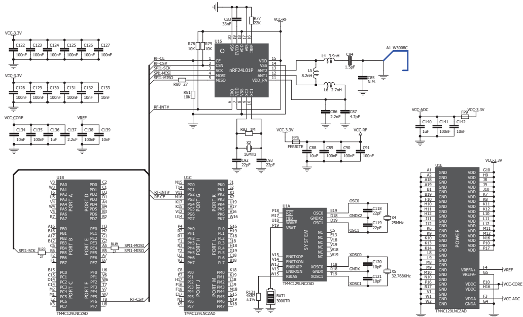
Figure 13-3: RF transceiver module connection schematic
