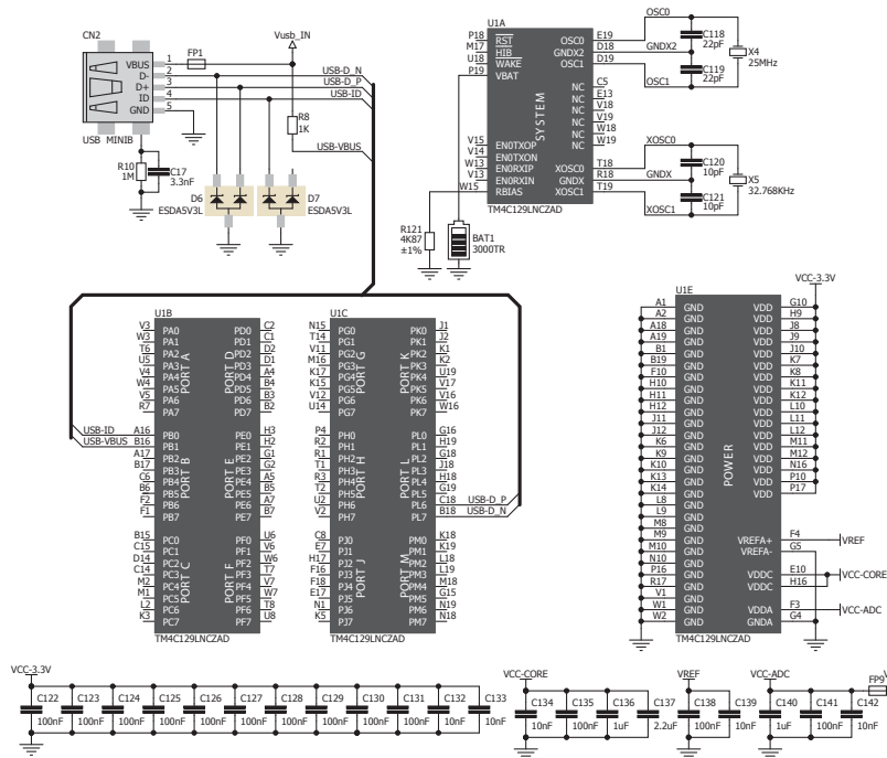
Figure 9-2: USB DEVICE module connection schematic
