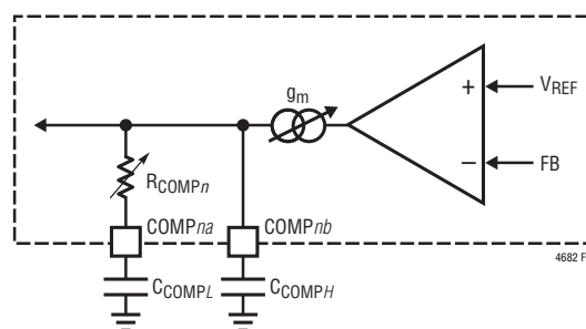
Figure 27. Programmable Loop Compensation
