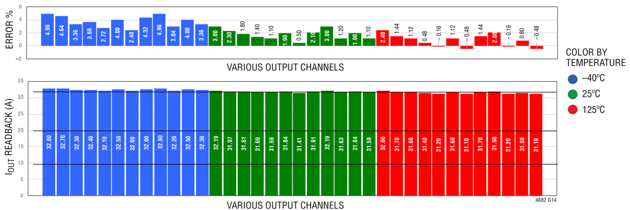
I_{OUT} READBACK AT 31.25A
