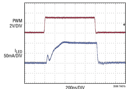
10,000:1 PWM Dimming at 100Hz
