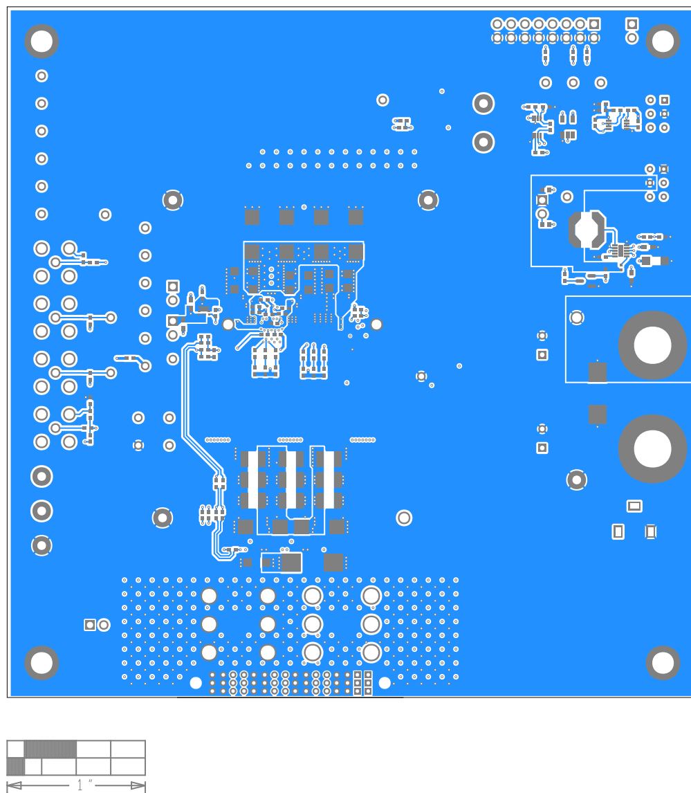
MAX20796 EV Kit PCB Layout—Bottom
