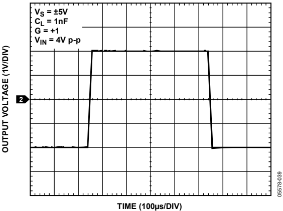
Figure 36. Large Signal Transient
