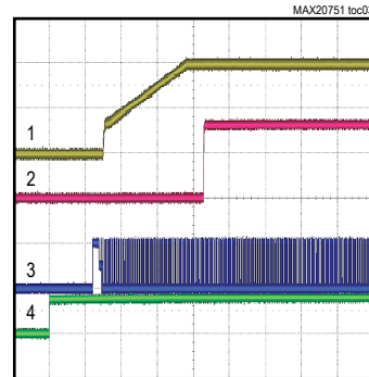
TURN-ON WAVEFORMS - NO LOAD
