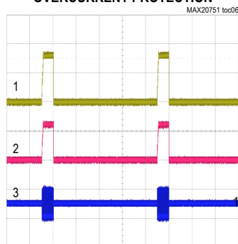
OUTPUT VOLTAGE IN HICCUP-MODE OVERCURRENT PROTECTION
