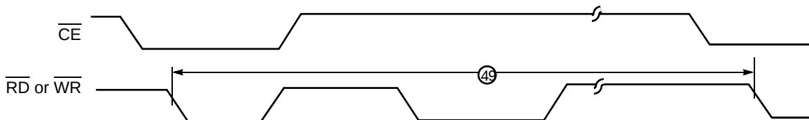
Figure 32. Z85230/L Cycle Timing Diagram
