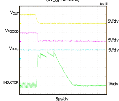
SHORT-CIRCUIT RESPONSE (5V OUT , 2.1MHz)
