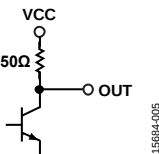
Figure 5. OUT Interface Schematic
