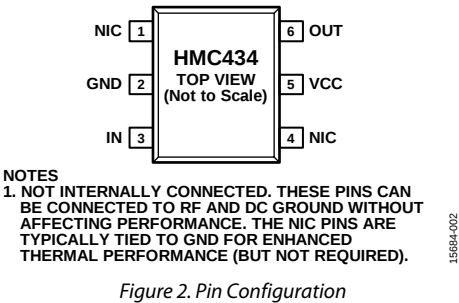
Figure 2. Pin Configuration
