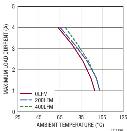
Figure 20. 12V IN to 36V OUT , 400kHz, Derating Curve, No Heat Sink
