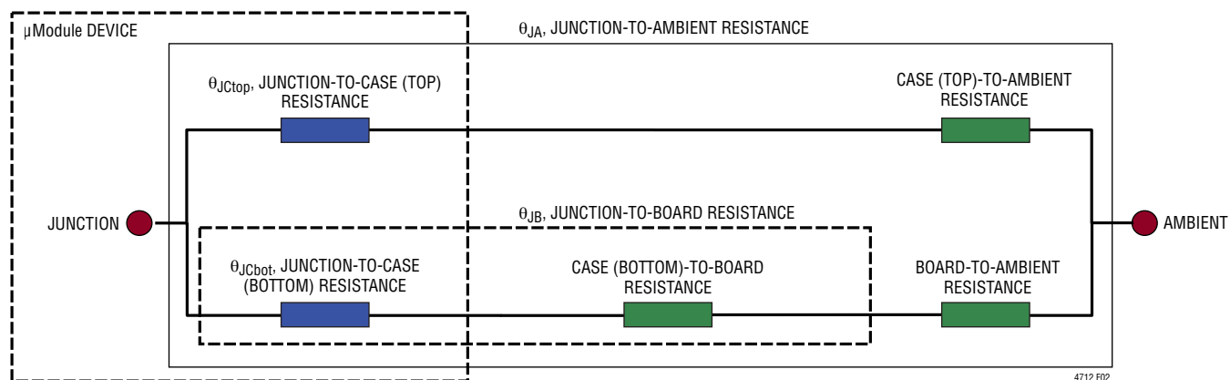
Figure 2. Graphical Representation of Thermal Coefficients, Including JESD51-12 Terms
