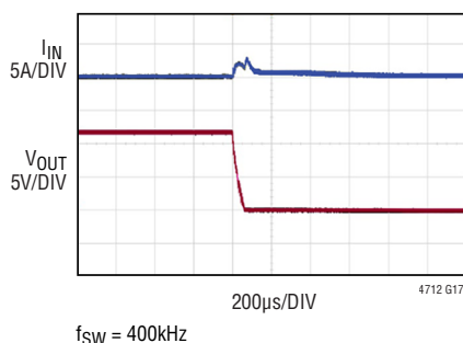
Short-Circuit with 12V IN to 12V OUT , No Load
