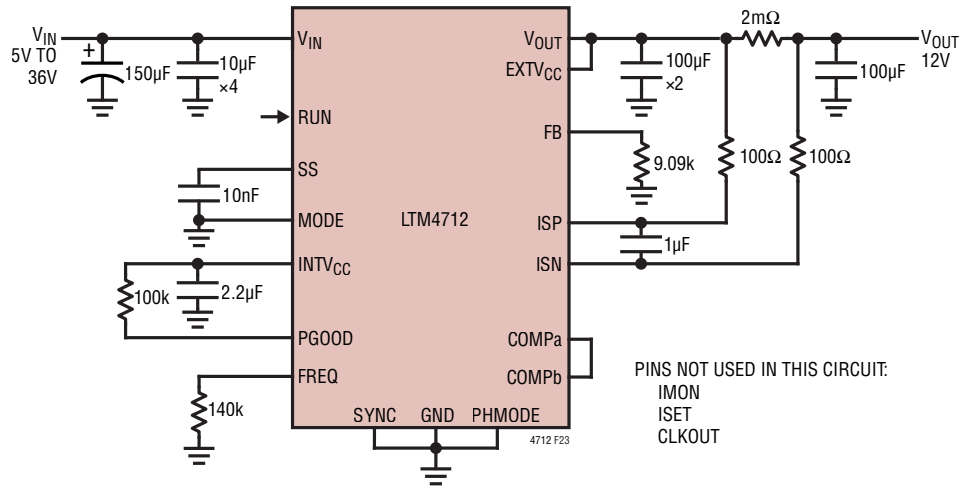
Figure 23. 12V OUT with Wide Input Voltage Range, 12A I OUT for Buck/Buck-Boost, 6A I OUT for Boost
