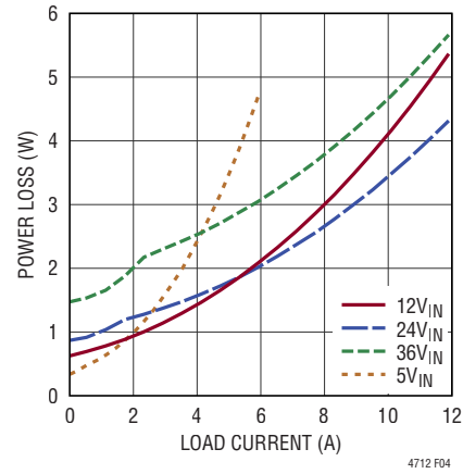
Figure 4. Power Loss 12V OUT , 400kHz, FCM
