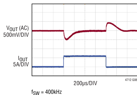
Transient Response, 12V IN to 12V OUT
