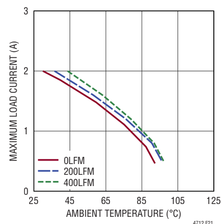
Figure 21. 5V IN to 36V OUT , 400kHz, Derating Curve, No Heat Sink
