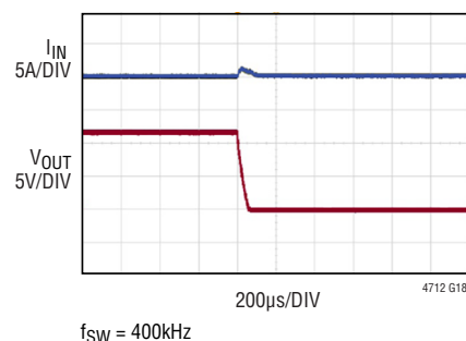
Short-Circuit with 36V IN to 12V OUT , No Load
