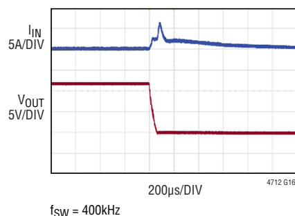
Short-Circuit with 5V IN to 12V OUT , No Load
