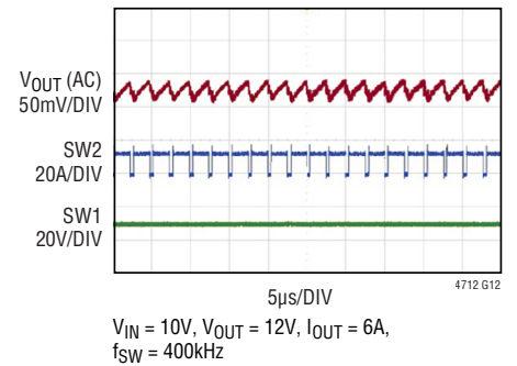
Switching Waveforms (Boost Region)
