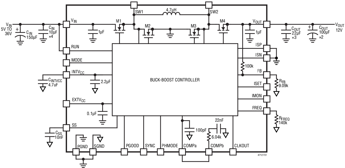
Figure 1. LTM4712 Block Diagram
