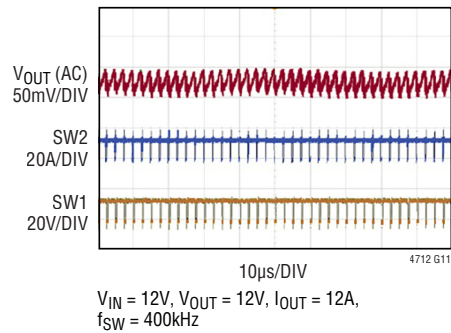
Switching Waveforms (Buck-Boost Region)
