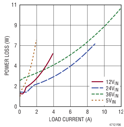
Figure 6. Power Loss 36V OUT , 400kHz, FCM
