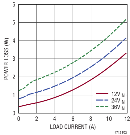
Figure 3. Power Loss 5V OUT , 400kHz, FCM
