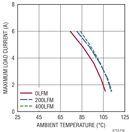
Figure 16. 12V IN to 24V OUT , 400kHz, Derating Curve, No Heat Sink
