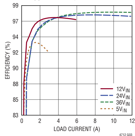
24V OUT Efficiency, 400kHz, FCM
