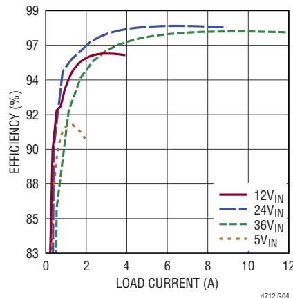
36V OUT Efficiency, 400kHz, FCM
