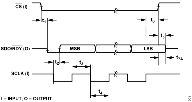
Figure 4. Read Cycle Timing Diagram (SDO and RDY Share a Pin with Bit SDO_RDYB_DLY Set)
