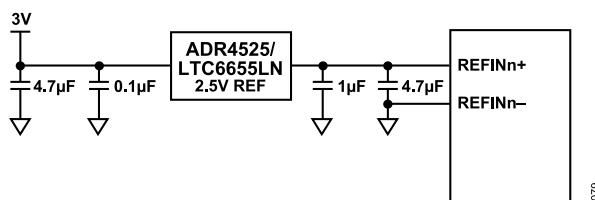
Figure 76. ADR4525/LTC6655LN-2.5 to AD4170-4 Connections
