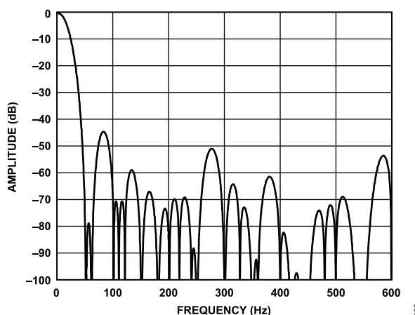
Figure 99. DC to 600 Hz, 16.667 SPS ODR, 60 ms Conversion Time Post Filter
