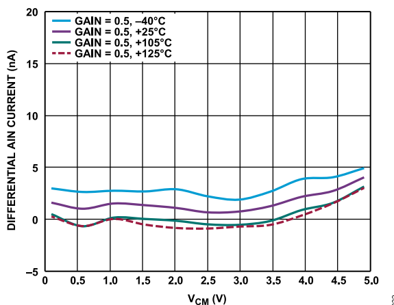
Figure 32. Differential AIN Current vs. V_{CM} ( V_{DIFF} = 0 V), Gain = 0.5
