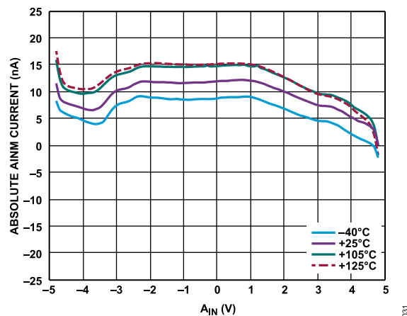
Figure 31. Absolute AINM Current vs. A_{IN} ( V_{CM} = (AVDD + AVSS)/2 ), Gain = 0.5
