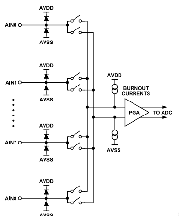
Figure 74. Analog Input Multiplexer Circuit
