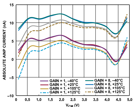
Figure 36. Absolute AINP Current vs. V_{CM} ( V_{DIFF} = 0 V), Gains of 1 and 8
