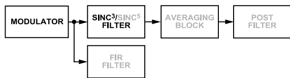
Figure 90. Sinc 3 Filter
