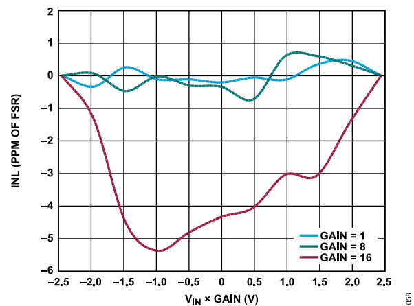
Figure 57. INL
