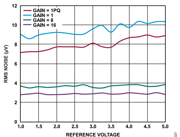
Figure 21. RMS Noise vs. Reference Voltage (Sinc 5 + Avg Filter, 125 kSPS)
