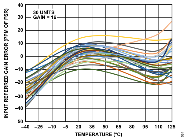
Figure 63. Input Referred Gain Error vs. Temperature (Gain = 16)
