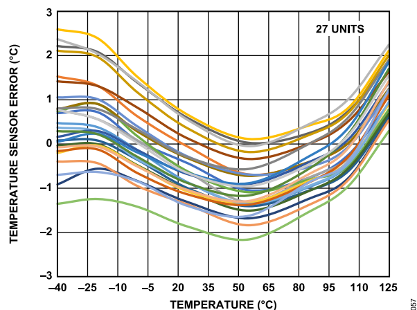
Figure 56. Internal Temperature Sensor Accuracy
