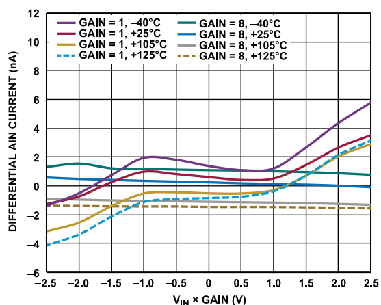
Figure 35. Differential AIN Current vs. V_{IN} ( V_{CM} = (AVDD + AVSS)/2 ), Gains of 1 and 8
