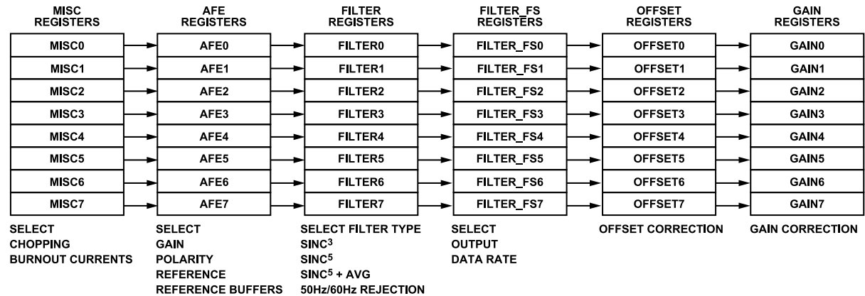
Figure 70. Setup Structure
