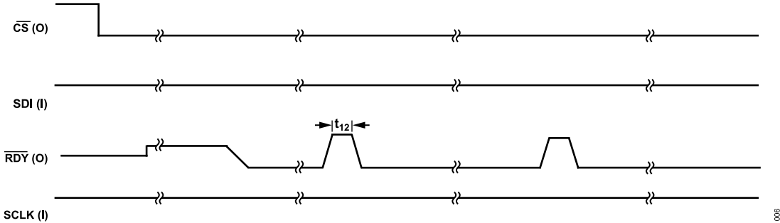
Figure 6. RDY High Time when RDY Is Initially Low and the Next Conversion is Available
