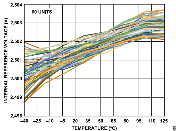
Figure 55. Internal Reference Voltage vs. Temperature (Soldered Devices)
