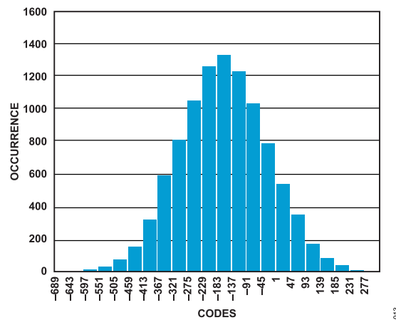
Figure 13. Noise Histogram ( \text{Sinc}^5 + Avg Filter, 125 kSPS, PGA_Gain = 16)
