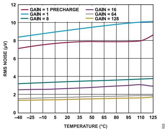
Figure 22. RMS Noise vs. Temperature ( \text{Sinc}^5 + Avg Filter, 125 kSPS, 2.5 V Reference)
