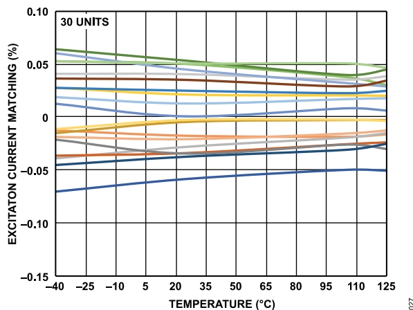
Figure 27. IOUTn Excitation Current Matching vs. Temperature (500 \mu\text{A} )
