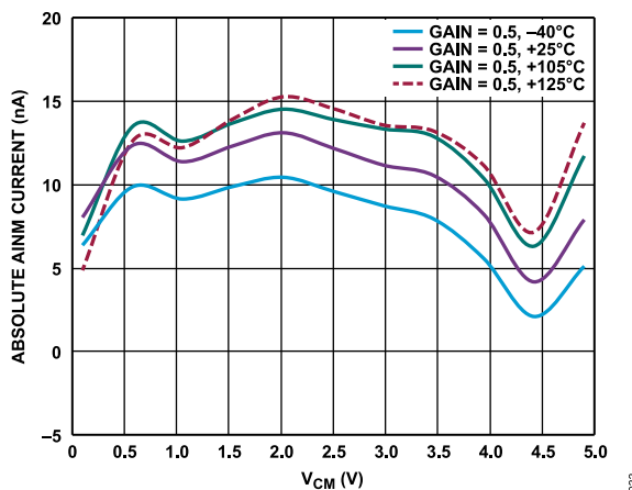
Figure 33. Absolute AINM Current vs. V_{CM} ( V_{DIFF} = 0 V), Gain = 0.5
