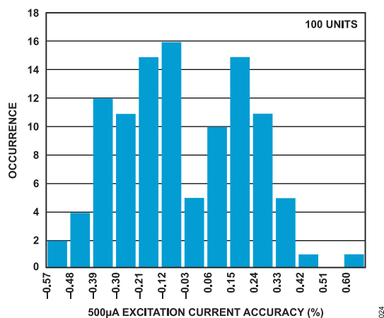
Figure 24. IOUTn Excitation Current Initial Accuracy (500 \mu\text{A} )
