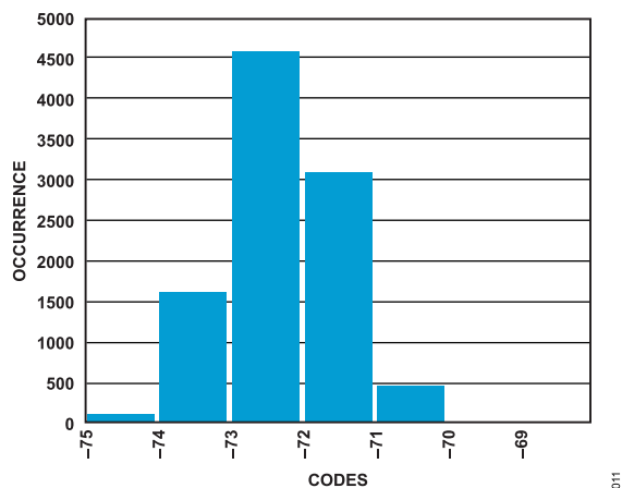
Figure 11. Noise Histogram ( \text{Sinc}^5 + Avg Filter, 50 SPS, PGA_Gain = 1)
