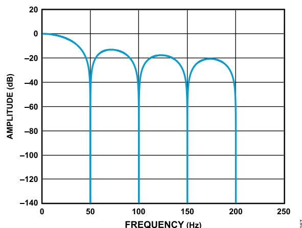
Figure 84. 50 Hz Rejection
