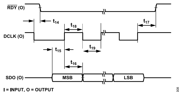
Figure 8. Continuous Transmit
