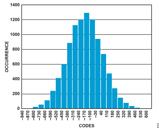
Figure 15. Noise Histogram (Default FIR Filter, 125 kSPS, PGA_Gain = 16)
