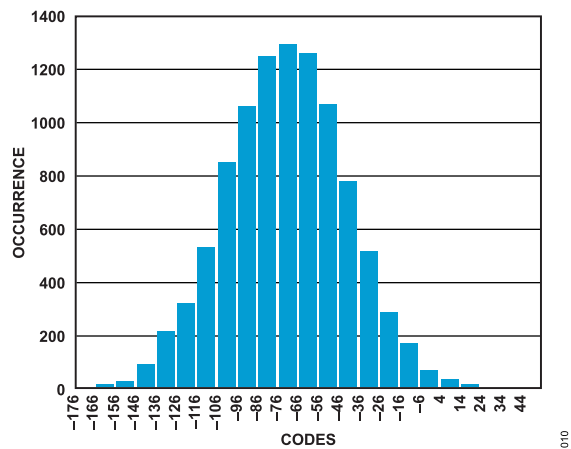
Figure 10. Noise Histogram ( \text{Sinc}^5 + Avg Filter, 125 kSPS, PGA_Gain = 1)
