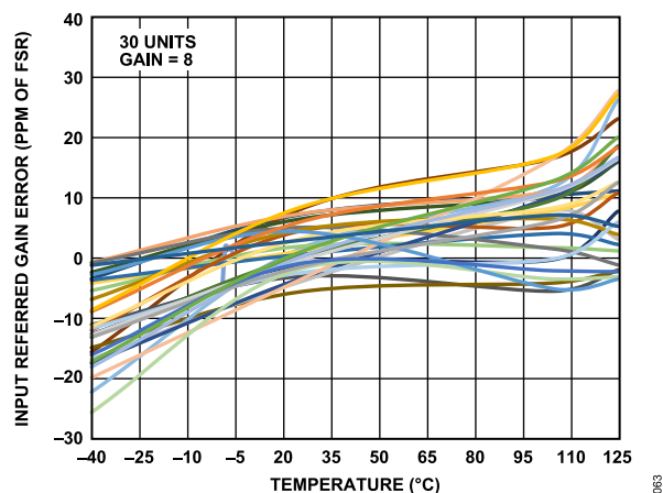
Figure 62. Input Referred Gain Error vs. Temperature (Gain = 8)
