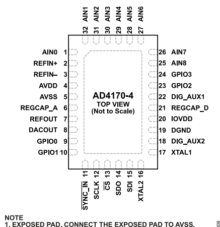
Figure 9. Pin Configuration
