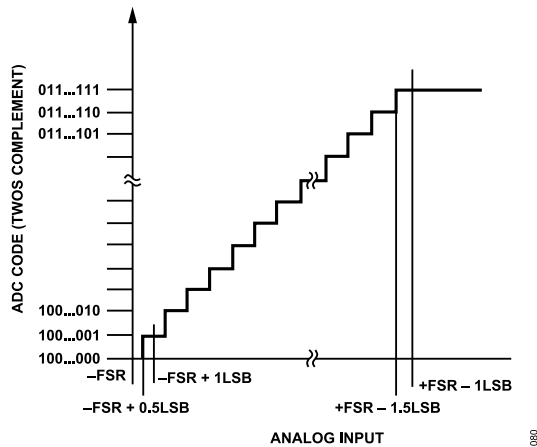
Figure 77. ADC Ideal Transfer Function (FS = full-scale)
