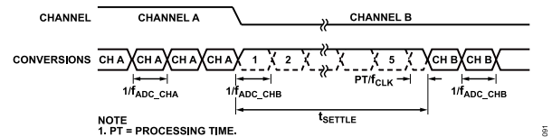
Figure 88. Sinc 5 Channel Change
