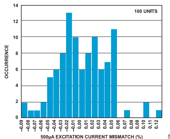
Figure 26. IOUTn Excitation Current Initial Matching (500 \mu\text{A} )
