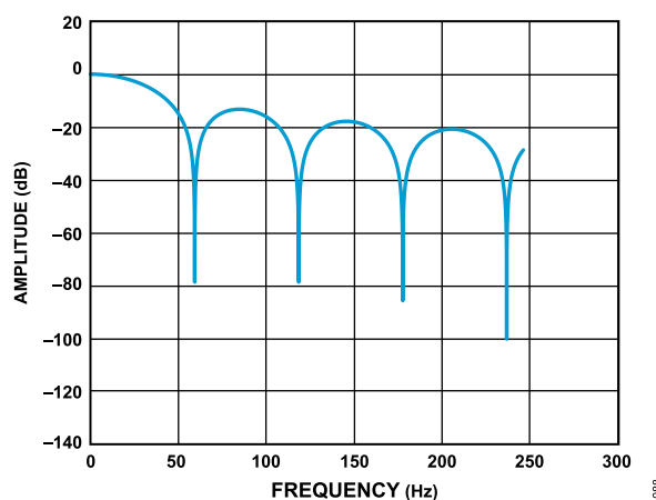
Figure 85. 60 Hz Rejection
