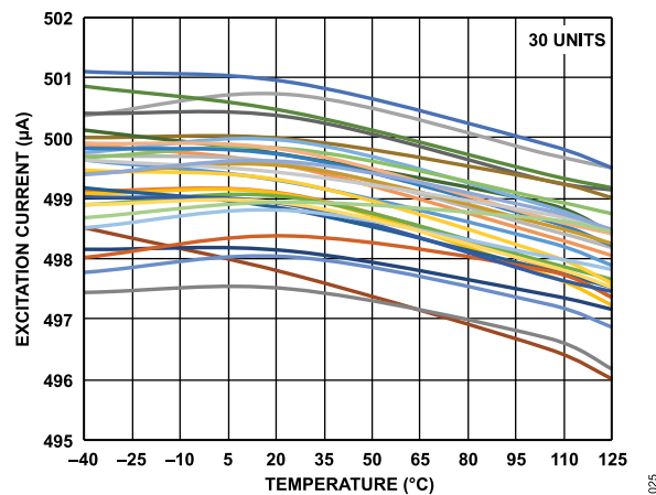
Figure 25. IOUTn Excitation Current vs. Temperature (500 \mu\text{A} )
