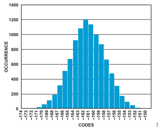
Figure 14. Noise Histogram ( \text{Sinc}^5 + Avg Filter, 50 SPS, PGA_Gain = 16)
