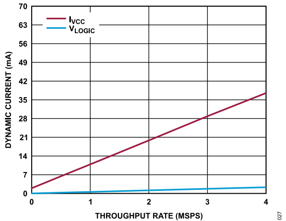
Figure 27. Dynamic Current vs. Throughput Rate
