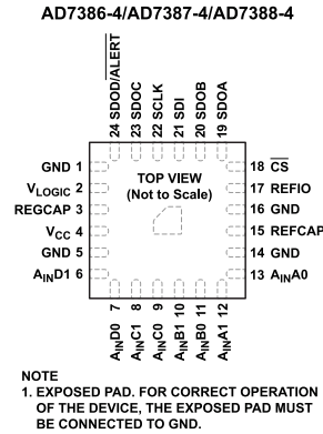
Figure 9. Pin Configuration
