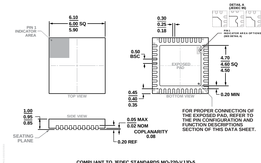
COMPLIANT TO JEDEC STANDARDS MO-220-VJJD-5 Figure 62. 40-Lead Lead Frame Chip Scale Package [LFCSP] 6 mm × 6 mm Body and 0.95 mm Package Height (CP-40-15) Dimensions shown in millimeters
