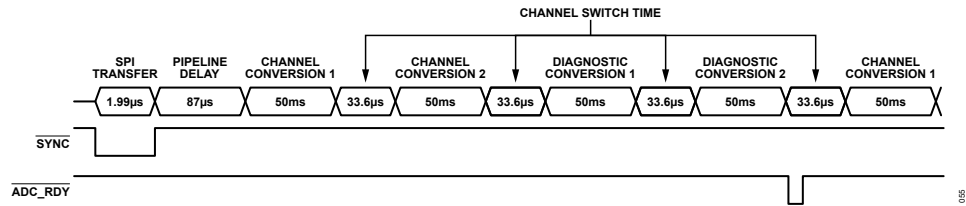
Figure 49. Multiple Measurements, Continuous Conversions Timing Diagram
