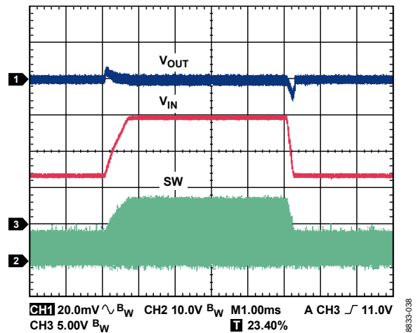
Figure 38. ADP2302 Line Transient, 7V to 15V, V_{OUT} = 3.3\text{ V} , I_{OUT} = 2\text{ A} , L = 6.8\ \mu\text{H} , C_{OUT} = 2 \times 22\ \mu\text{F}
