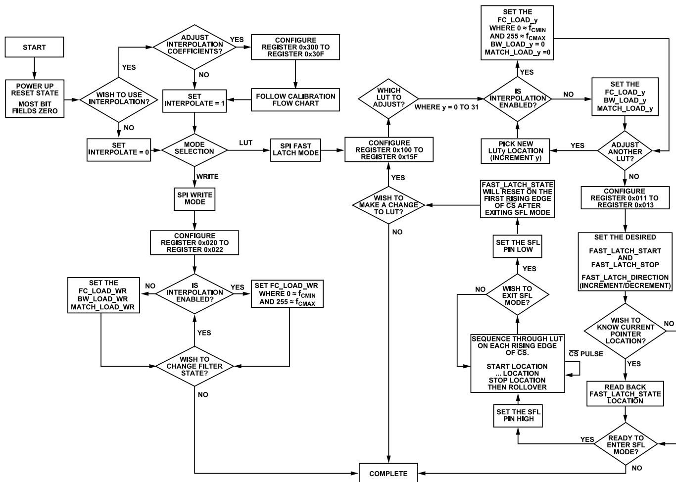
Figure 25. Programming Flow Chart
