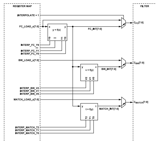
Figure 21. Interpolation Diagram
