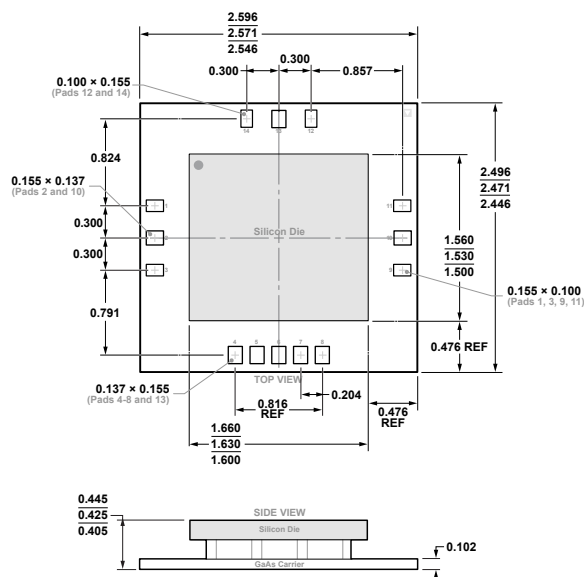
Figure 20. 14-Pad Die on Carrier [CHIP], (C-14-8), Dimensions shown in millimeters
