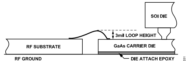
Figure 19. Bonding Diagram Side View
