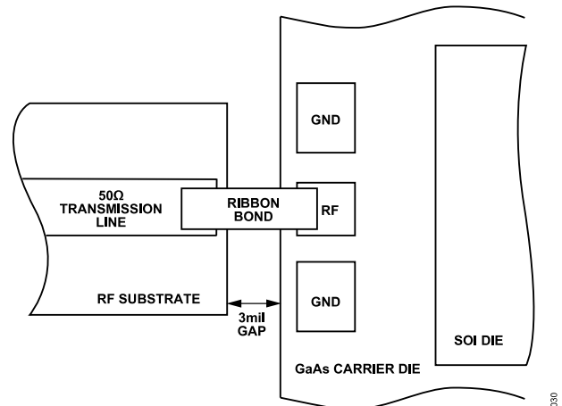
Figure 18. Bonding Diagram Top View
