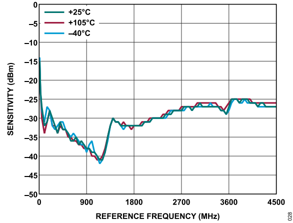
Figure 28. Reference Sensitivity for DMA Buffer at Various Temperatures
