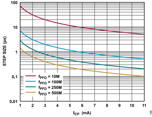
Figure 46. Bleed Current Delay Step Size
