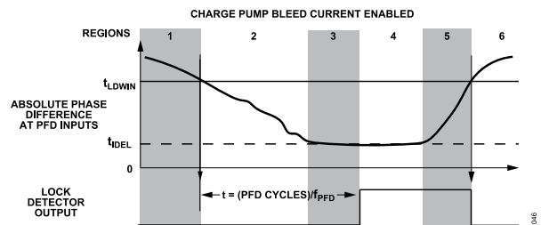
Figure 48. Lock Detector Timing, Bleed Current Enabled
