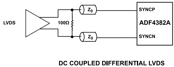
Figure 68. DC-Coupled Differential LVDS (Set SYNC_SEL = 1)
