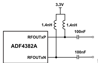
Figure 58. RFOUT Interface Schematic
