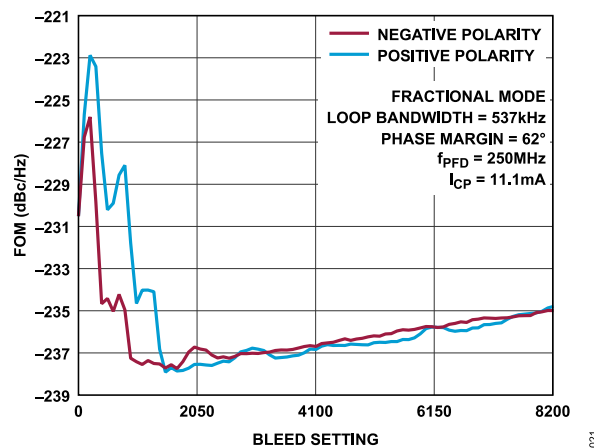
Figure 21. FOM, L_{NORM} Fractional Mode vs. Bleed Setting, f_{PFD} = 250 MHz, R_{FOUT} = 20.001 GHz
