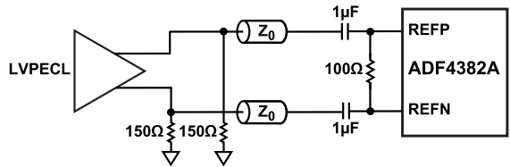
Figure 63. Differential, Low Voltage, Positive Emitter-Coupled Logic (LVPECL)
