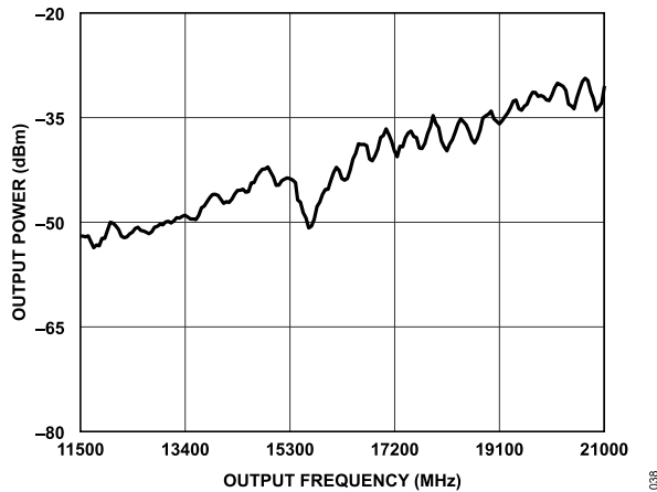
Figure 39. Output Power when Buffer Powered Down (PD_RFOUTx = 1) vs. Output Frequency
