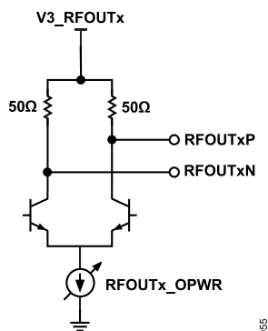
Figure 57. Simplified RF Output Buffer Schematic
