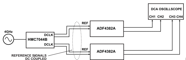
Figure 71. EZSync Configuration
