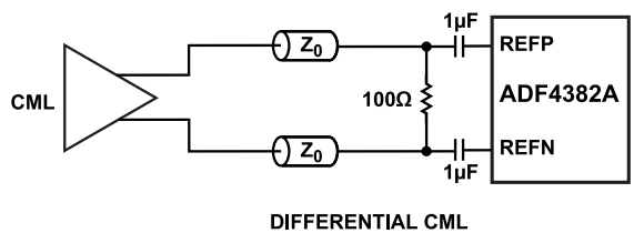
Figure 65. Differential CML
