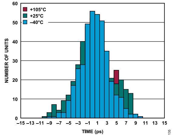
Figure 35. Normalized Propagation Delay ( t_{PD} ) Histogram
