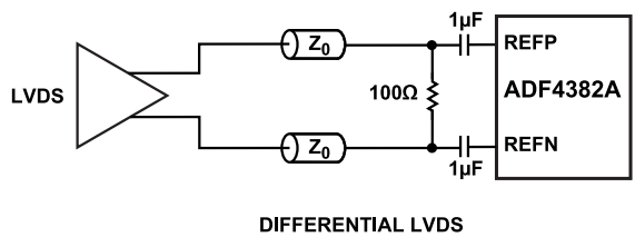
Figure 64. Differential LVDS
