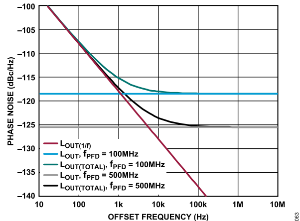
Figure 70. Theoretical In-Band Phase Noise, f_{OUT} = 10 GHz
