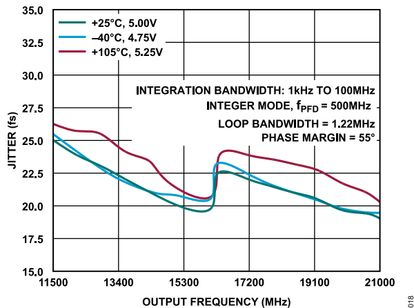
Figure 18. 1 kHz to 100 MHz Integrated Jitter in Integer Mode, f_{PFD} = 500 \text{ MHz}
