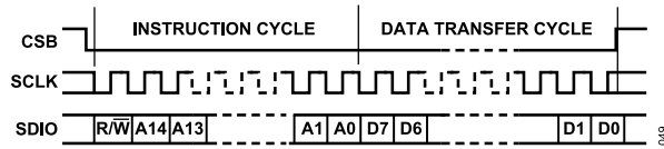
Figure 51. Serial Interface, MSB First (LSB_FIRST = 0)
