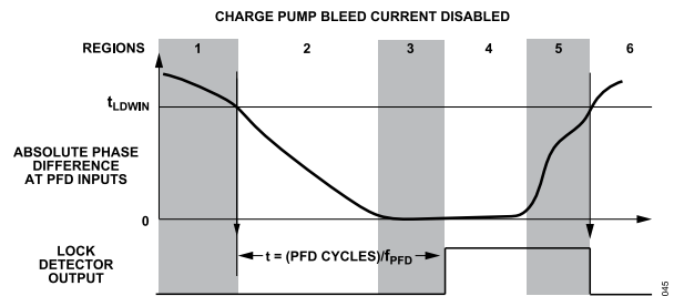
Figure 47. Lock Detector Timing, Bleed Current Disabled
