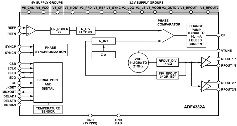
Figure 42. PLL Loop Diagram
