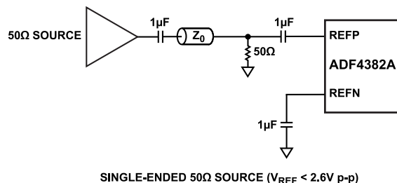
Figure 60. Single-Ended 50 \Omega Source ( V_{\text{REF}} < 2.6 \text{ V p-p} )
