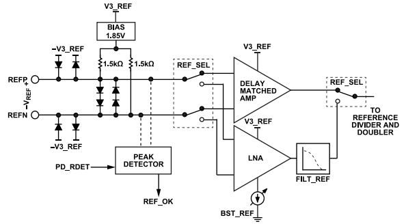
Figure 43. Reference Input Stage
