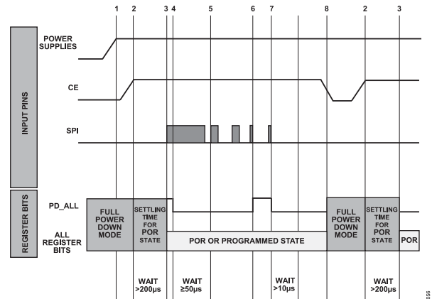
Figure 59. Power-Up and Initialization
