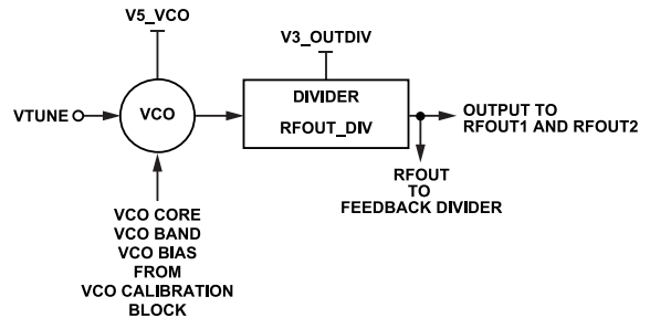
Figure 53. VCO and Clock Output Divider
