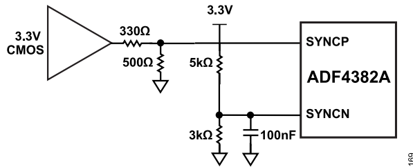
Figure 69. DC-Coupled 3.3 V Single-Ended Logic to LVDS Input (Set SYNC_SEL = 1)
