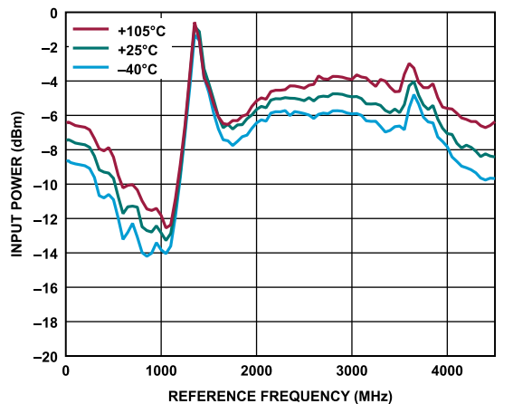
Figure 27. Minimum Input Signal for REF_OK = 1 for LNA Buffer at Various Temperatures
