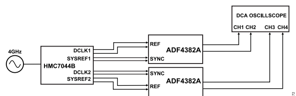
Figure 72. Timed Synchronization Configuration
