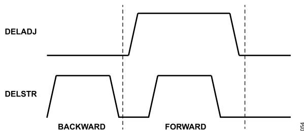
Figure 56. DELSTR and DELADJ Timing Diagrams
