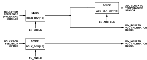
Figure 54. VCO Calibration Dividers
