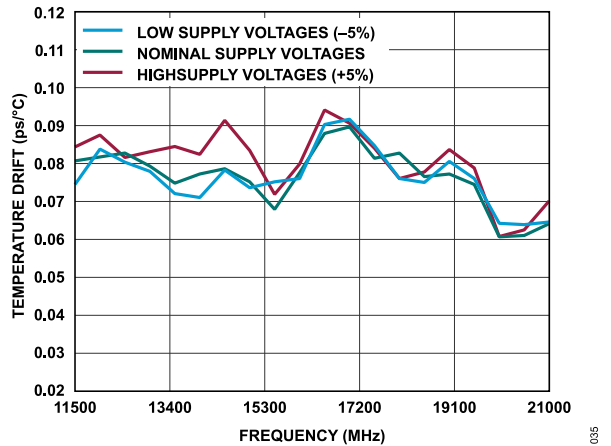
Figure 36. Temperature Drift vs. Frequency
