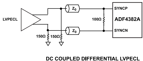
Figure 67. DC-Coupled Differential LVPECL (Set SYNC_SEL = 0)
