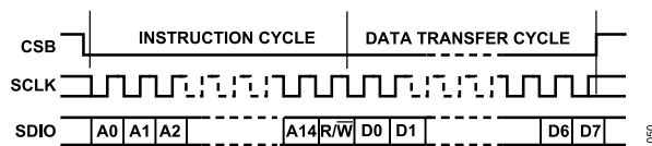
Figure 52. Serial Interface, LSB First (LSB_FIRST = 1)
