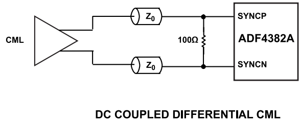
Figure 66. DC-Coupled Differential CML (Set SYNC_SEL = 0)
