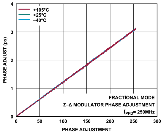
Figure 38. Phase Shift vs. PHASE_ADJUSTMENT for Various Temperatures
