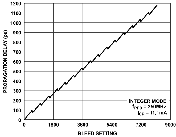
Figure 37. Propagation Delay vs. Bleed Setting
