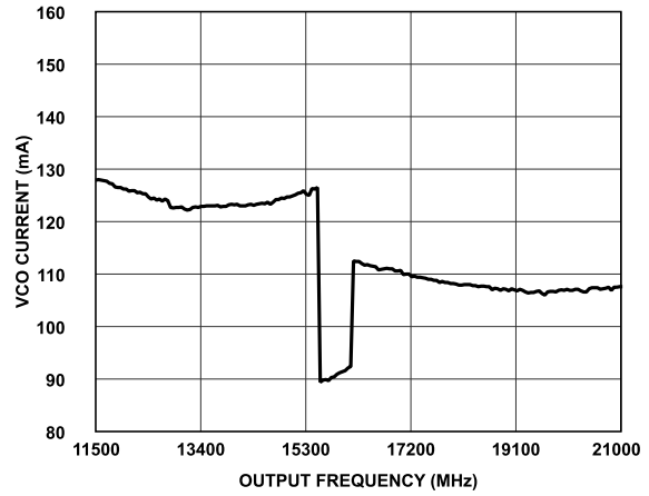
Figure 40. VCO Current vs. Output Frequency
