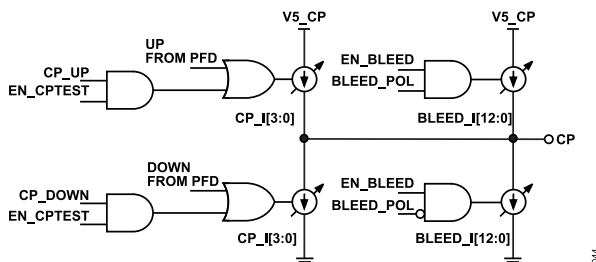
Figure 45. Simplified Charge Pump Schematic
