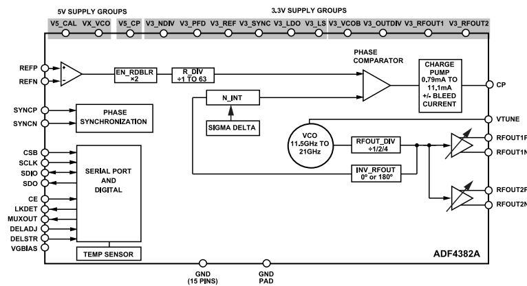
Figure 1. ADF4382A Functional Block Diagram
