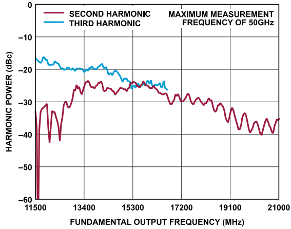
Figure 25. Harmonic Power vs. Fundamental Output Frequency
