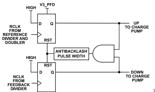
Figure 44. Simplified PFD Schematic
