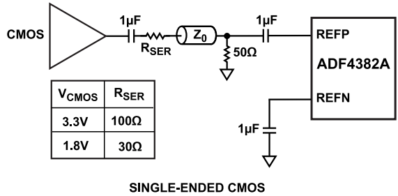
Figure 62. Single-Ended CMOS ( R_{SER} Is the Series Resistance.)
