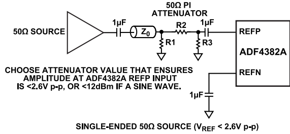
Figure 61. Single-Ended 50 Ω Source ( V_{REF} < 2.6 V\text{ p-p}</math>)
