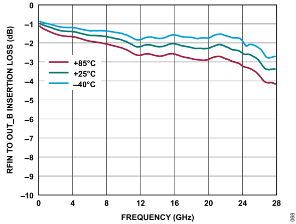
Figure 70. RFIN to OUT_B Insertion Loss vs. Frequency Over Temperature, 100 MHz to 28 GHz, Mode = External Bypass B
