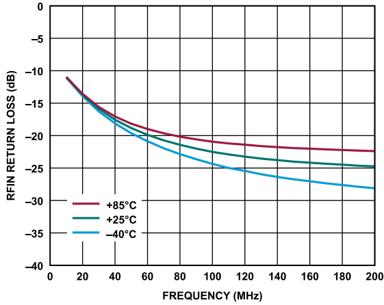
Figure 18. RFIN Return Loss vs. Frequency Over Temperature, 10 MHz to 200 MHz, V_{DD} = 8.5\text{ V} , I_{DQ} = 90\text{ mA} , Mode = Internal Amplifier
