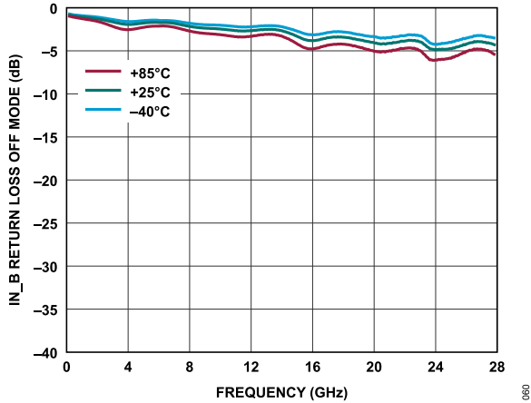
Figure 62. IN_B Return Loss Off Mode vs. Frequency Over Temperature, 100 MHz to 28 GHz, Mode = External Bypass A
