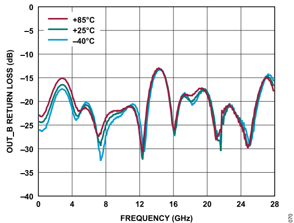
Figure 72. OUT_B Return Loss vs. Frequency Over Temperature, 100 MHz to 28 GHz, Mode = External Bypass B
