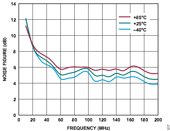
Figure 20. Noise Figure vs. Frequency Over Temperature, 10 MHz to 200 MHz, V_{DD} = 8.5\text{ V} , I_{DQ} = 90\text{ mA} , Mode = Internal Amplifier
