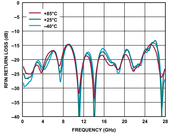
Figure 21. RFIN Return Loss vs. Frequency Over Temperature, 200 MHz to 28 GHz, V_{DD} = 8.5\text{ V} , I_{DQ} = 90\text{ mA} , Mode = Internal Amplifier
