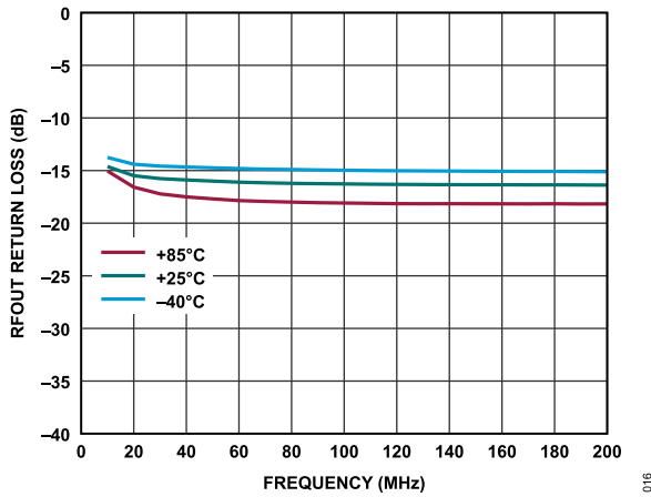
Figure 19. RFOUT Return Loss vs. Frequency Over Temperature, 10 MHz to 200 MHz, V_{DD} = 8.5\text{ V} , I_{DQ} = 90\text{ mA} , Mode = Internal Amplifier
