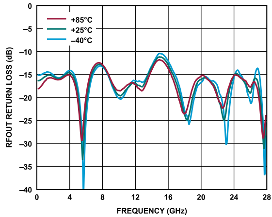
Figure 22. RFOUT Return Loss vs. Frequency Over Temperature, 200 MHz to 28 GHz, V_{DD} = 8.5\text{ V} , I_{DQ} = 90\text{ mA} , Mode = Internal Amplifier
