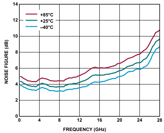
Figure 23. Noise Figure vs. Frequency Over Temperature, 200 MHz to 28 GHz, V_{DD} = 8.5\text{ V} , I_{DQ} = 90\text{ mA} , Mode = Internal Amplifier
