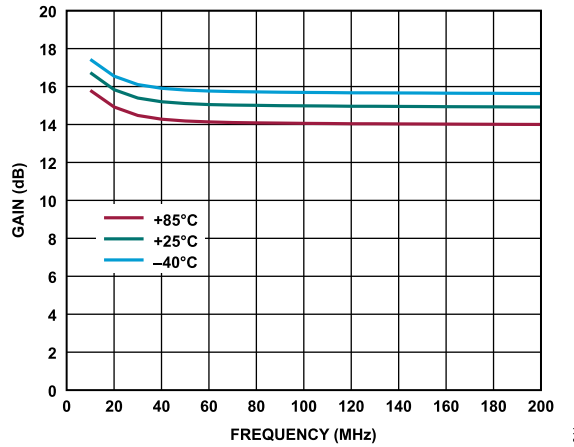
Figure 13. Gain vs. Frequency Over Temperature, 10 MHz to 200 MHz, V_{DD} = 8.5 V, I_{DQ} = 90 mA, Mode = Internal Amplifier
