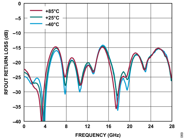
Figure 71. RFOUT Return Loss vs. Frequency Over Temperature, 100 MHz to 28 GHz, Mode = External Bypass B
