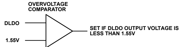
Figure 121. Digital LDO Monitor
