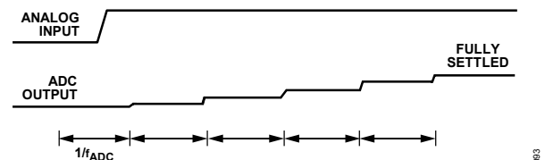
Figure 83. Asynchronous Step Change in the Analog Input
