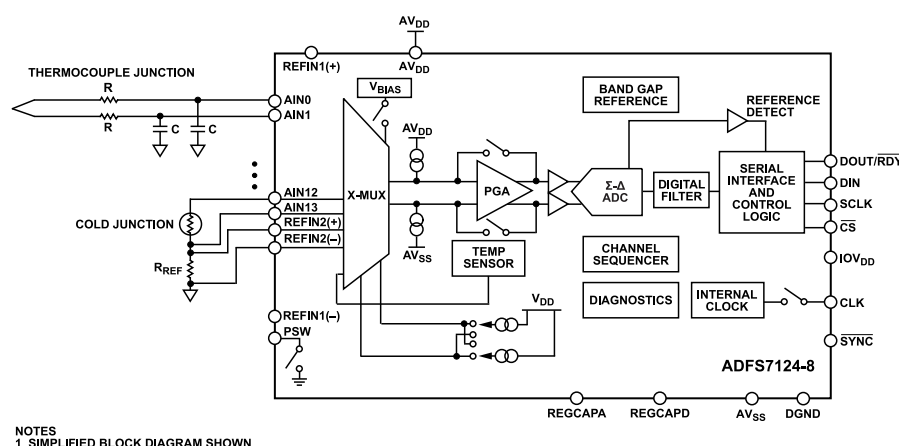
Figure 126. Thermocouple Application
