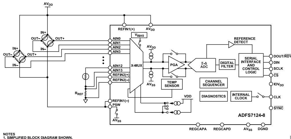
Figure 64. Basic Connection Diagram
