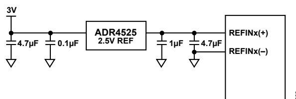
Figure 76. ADR4525 to ADFS7124-8 Connections
