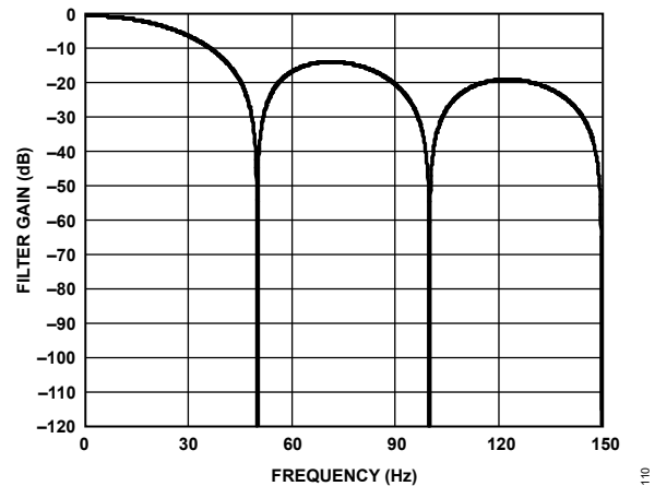
Figure 100. 50 Hz Rejection
