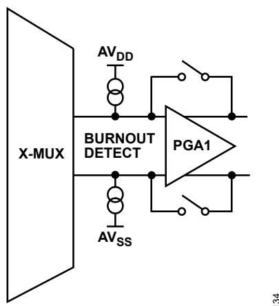
Figure 124. Burnout Currents
