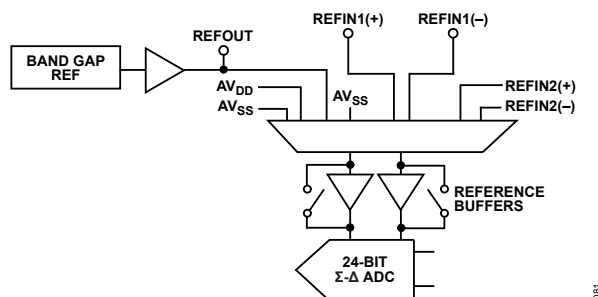
Figure 75. Reference Connections
