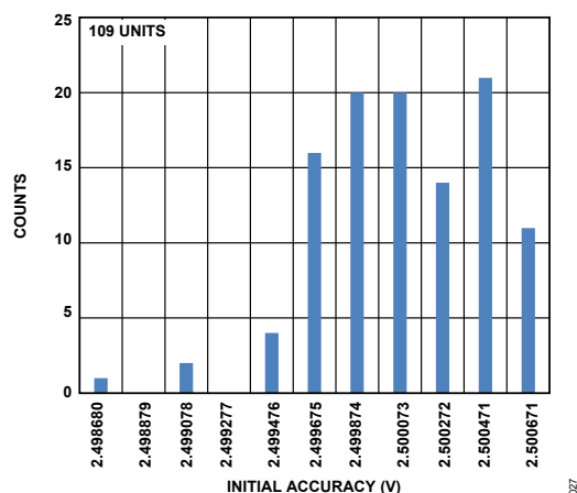
Figure 28. Internal Reference Voltage Histogram
