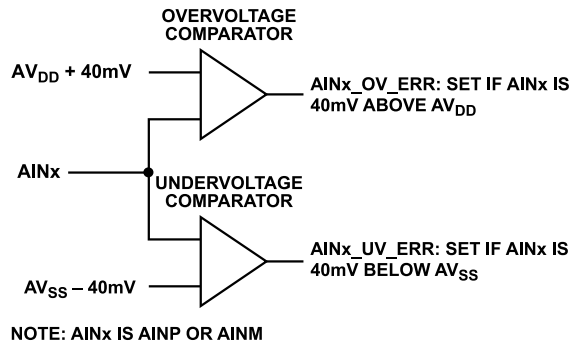
Figure 119. Analog Input Overvoltage/Undervoltage Monitors
