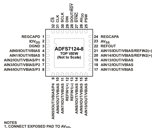
Figure 9. Pin Configuration
