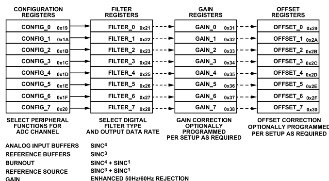
Figure 69. ADC Setup Register Grouping
