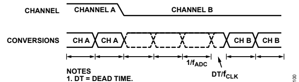
Figure 90. Sinc 3 Channel Change
