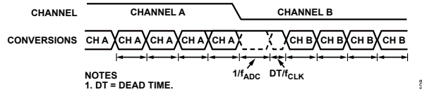
Figure 98. Fast Settling, \text{Sinc}^4 + \text{Sinc}^1 Filter
