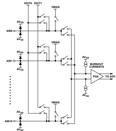
Figure 77. Excitation Current and Bias Voltage Connections
