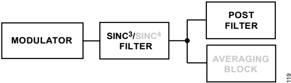
Figure 109. Post Filters
