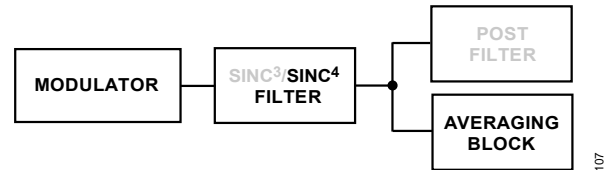
Figure 97. Fast Settling Mode, Sinc 4 + Sinc 1 Filter
