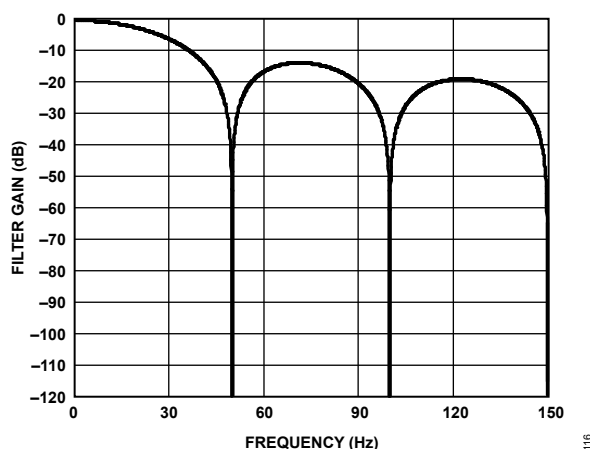
Figure 106. 50 Hz Rejection
