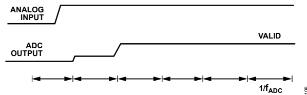
Figure 99. Step Change on the Analog Input, \text{Sinc}^4 + \text{Sinc}^1 Filter
