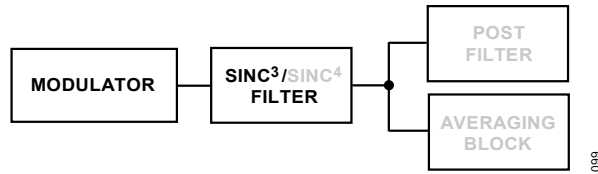
Figure 89. Sinc 3 Filter
