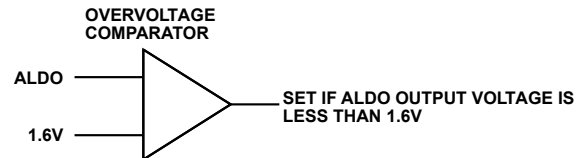
Figure 120. Analog LDO Monitor
