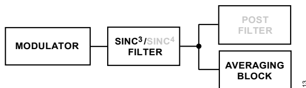
Figure 103. Fast Settling Mode, Sinc 3 + Sinc 1 Filter
