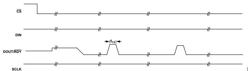
Figure 7. \overline{DOUT}/\overline{RDY} High Time when \overline{DOUT}/\overline{RDY} is Initially Low and the Next Conversion is Available
