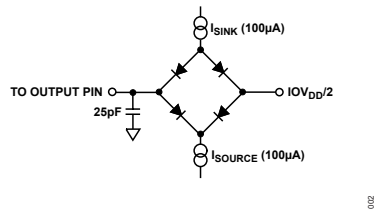
Figure 2. Load Circuit for Timing Characterization
