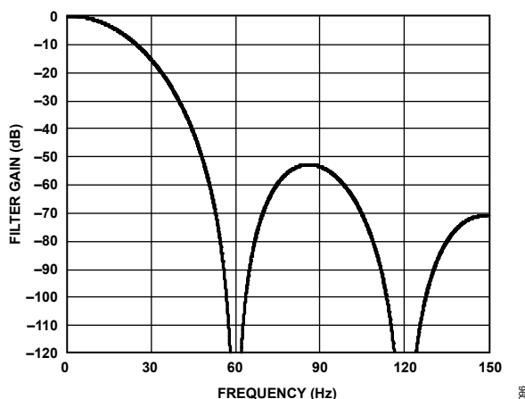
Figure 86. \text{sinc}^4 Filter Response (60 SPS Output Data Rate, Zero Latency Disabled or 15 SPS Output Data Rate, Zero Latency Enabled)
