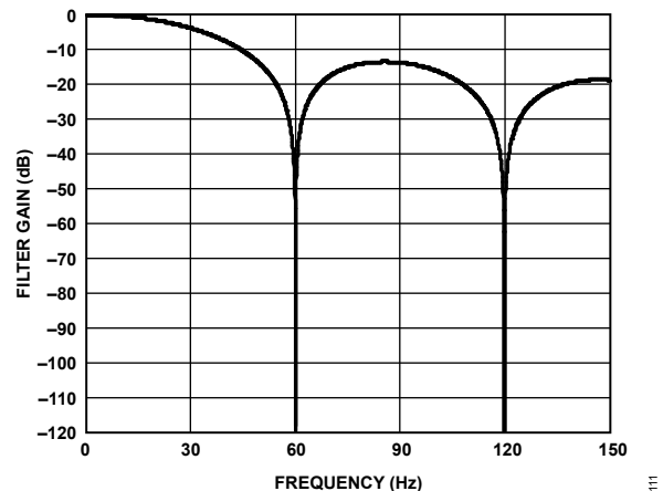
Figure 101. 60 Hz Rejection
