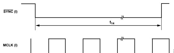
Figure 8. \overline{SYNC} Pulse Width
