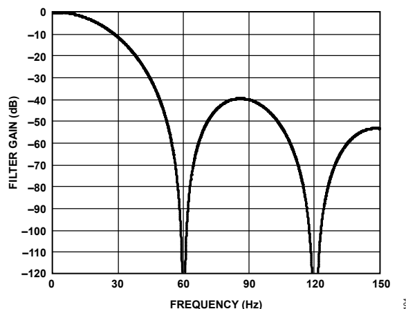
Figure 94. Sinc 3 Filter Response (60 SPS Output Data Rate, Zero Latency Disabled or 20 SPS Output Data Rate, Zero Latency Enabled)
