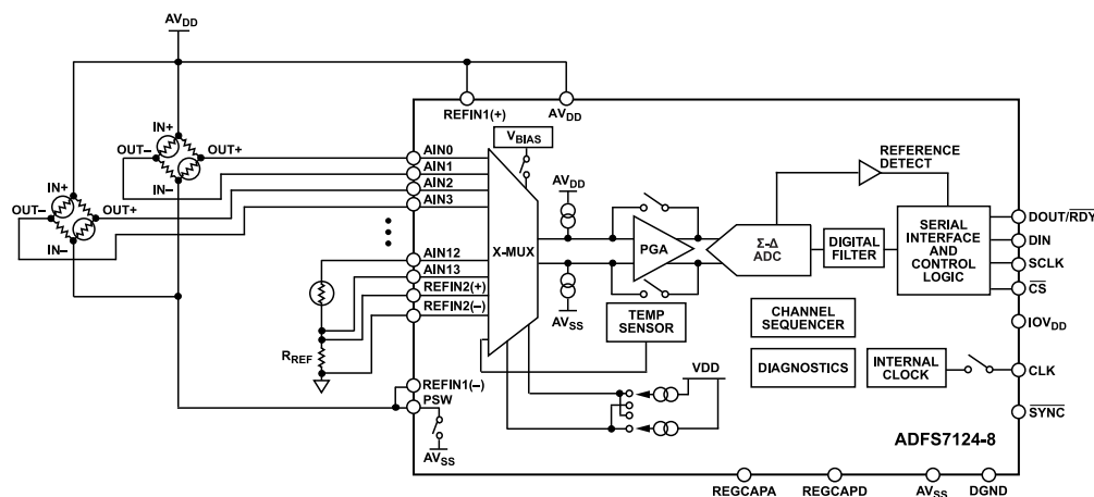
Figure 128. Flowmeter Application
