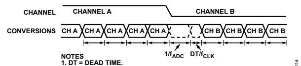
Figure 104. Fast Settling, Sinc 3 + Sinc 1 Filter
