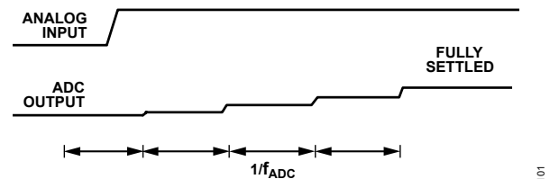
Figure 91. Asynchronous Step Change in the Analog Input
