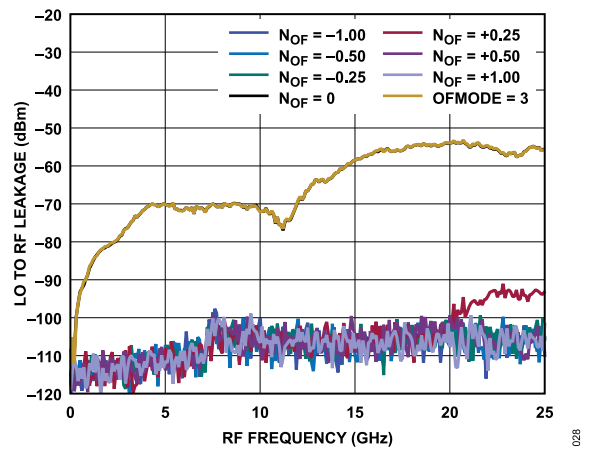
Figure 33. LO to RF Leakage for LOMODE = 2, Measurement Frequency = f_{RF}/2 + N_{OF} \times f_{OF} for OFMODE = 2, and f_{RF}/2 + f_{IF} for OFMODE = 3
