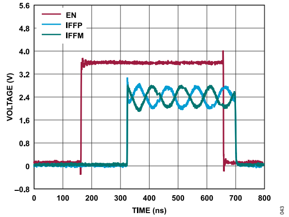
Figure 43. Turn-On/Off Time with Continuous Wave RF = 1 GHz, 10 dBm, IF = 10 MHz, 50 \Omega Load at IFFP and IFFM
