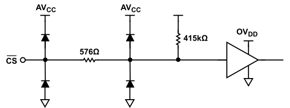
Figure 68. SPI Chip Select Interface
