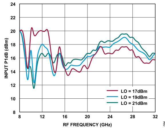
Figure 80. Input P1dB vs. RF Frequency at Various LO Power Levels, TA = 25°C
