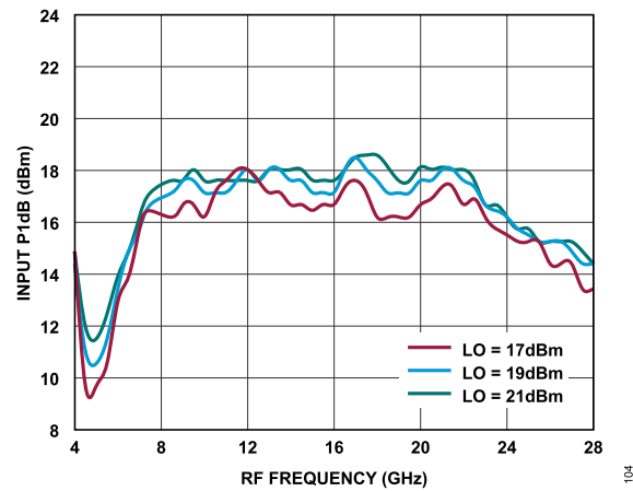
Figure 88. Input P1dB vs. RF Frequency at Various LO Power Levels, T_A = 25^{\circ}\text{C}
