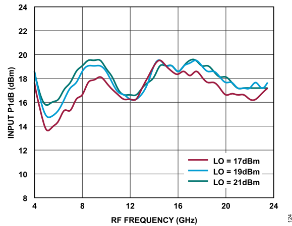
Figure 104. Input P1dB vs. RF Frequency at Various LO Power Levels, T_A = 25^\circ\text{C}
