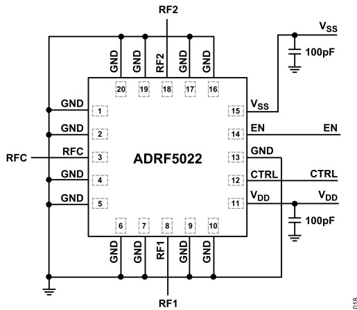
Figure 18. Recommended Schematic
