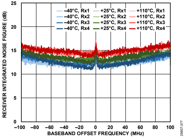
Figure 448. Receiver Integrated Noise Figure vs. Baseband Offset Frequency, 200 MHz Bandwidth, Sample Rate = 245.76 MSPS, Integrated in 200 kHz Steps
