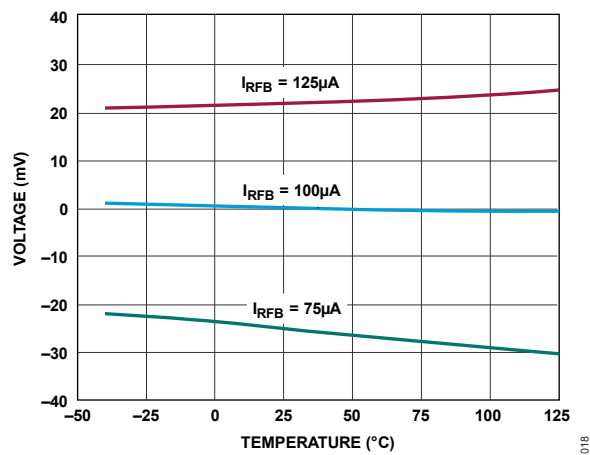
Figure 19. (R_{FB} - V_{IN}) Voltage
