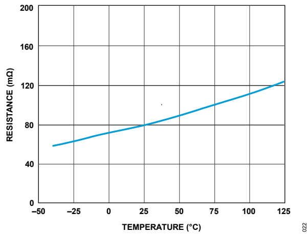
Figure 23. R_{DS(ON)}
