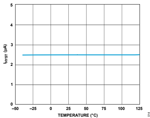
Figure 15. EN/UVLO Hysteresis Current
