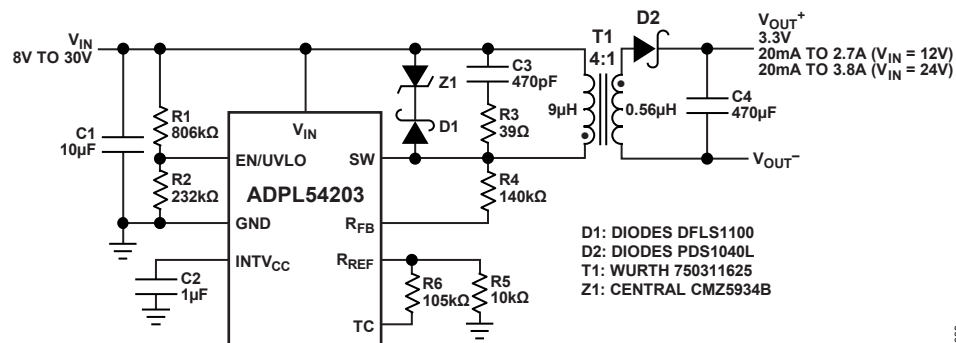
Figure 35. 8V to 30V IN /3.3V OUT Isolated Flyback Converter
