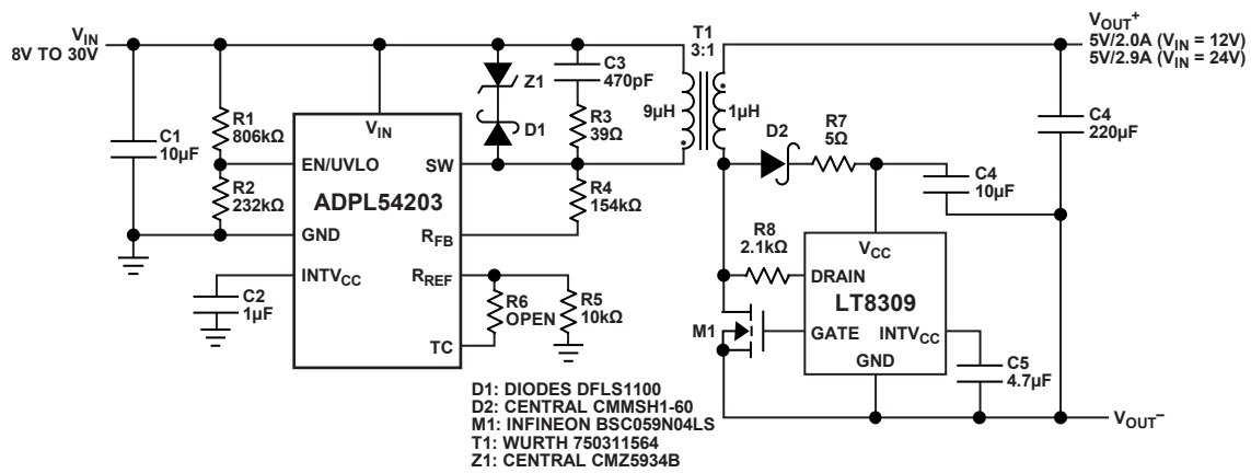
Figure 40. 8V to 30V IN /5V OUT Isolated Flyback Converter with LT8309
