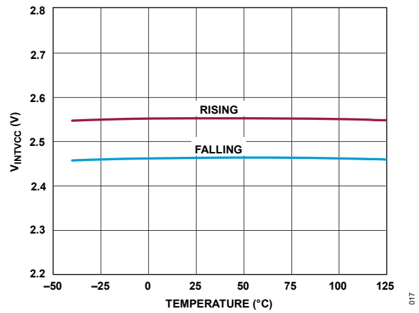
Figure 18. INTV_{CC} UVLO Threshold
