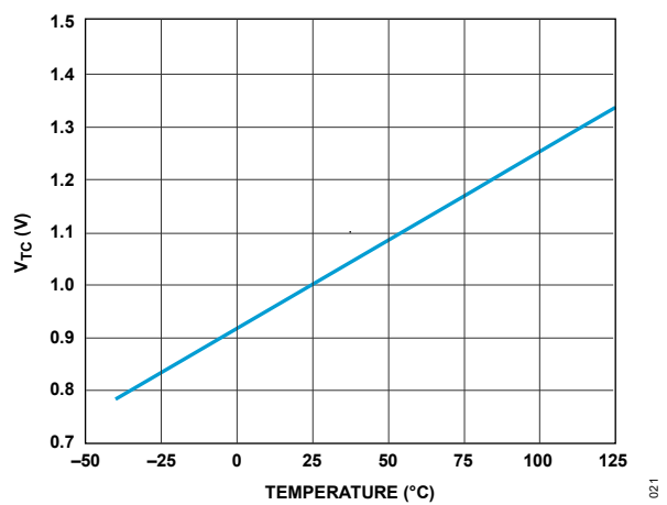
Figure 22. TC Pin Voltage
