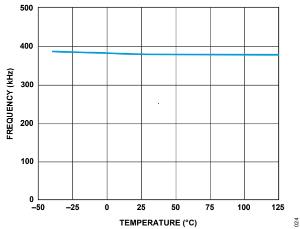
Figure 25. Maximum Switching Frequency
