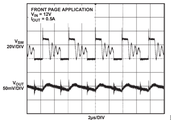
Figure 9. Discontinuous Mode Waveforms
