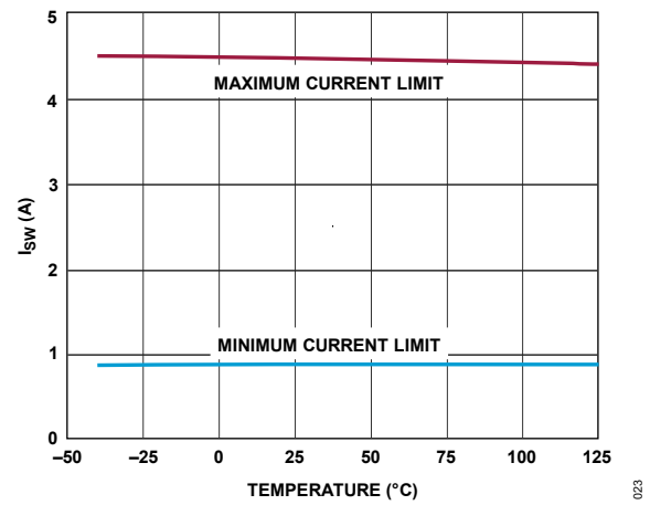
Figure 24. Switch Current Limit
