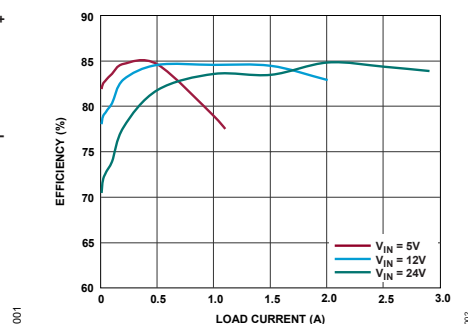
Figure 2. Efficiency vs. Load Current
