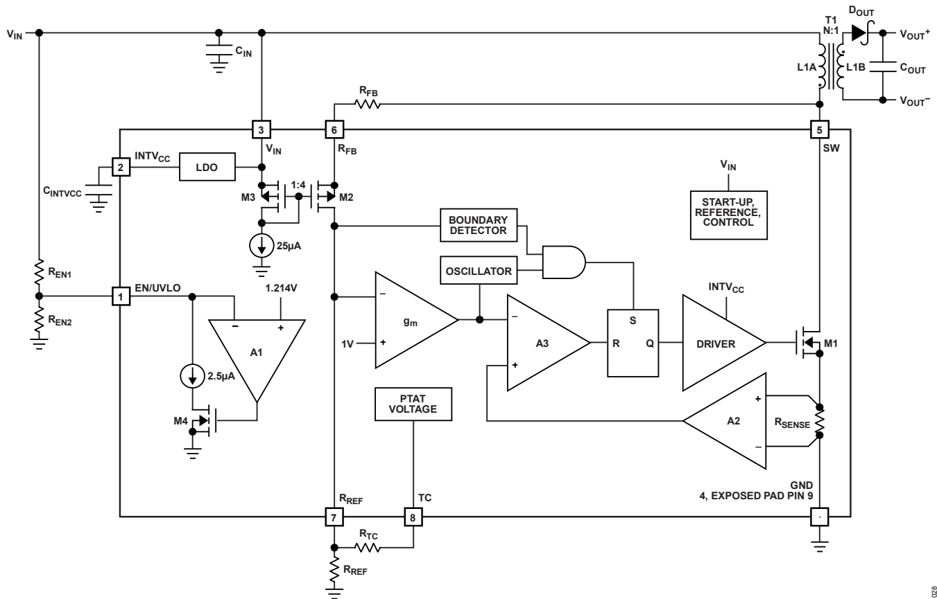
Figure 4. BLOCK DIAGRAM
