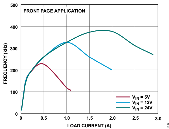
Figure 7. Switching Frequency vs. Load Current
