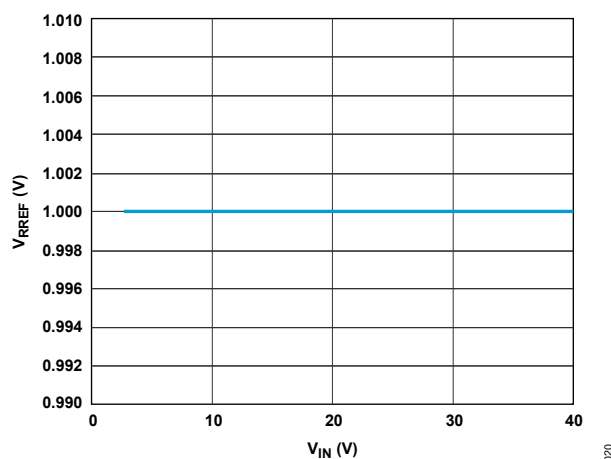
Figure 21. R_{REF} Line Regulation
