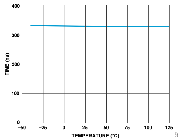
Figure 28. Minimum Switch-Off Time
