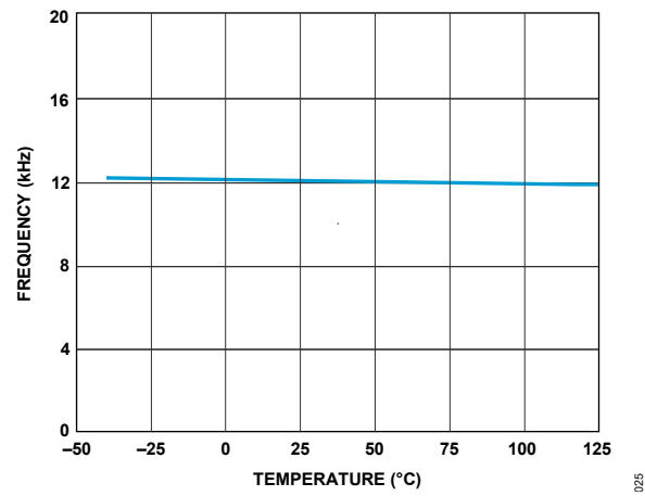
Figure 26. Minimum Switching Frequency
