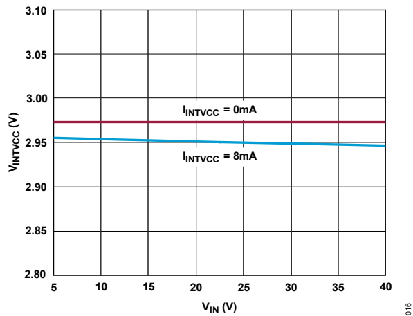
Figure 17. INTV_{CC} Voltage vs. V_{IN}
