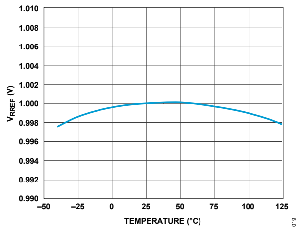
Figure 20. R_{REF} Regulation Voltage
