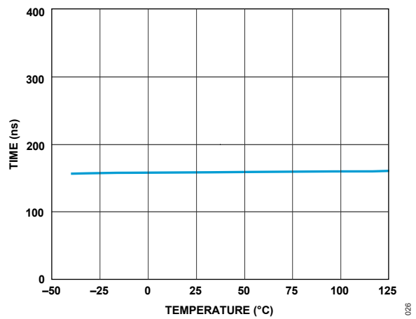
Figure 27. Minimum Switch-On Time
