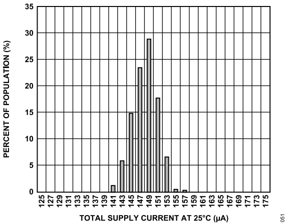
Figure 25. Total Supply Current at 25°C, 3.3 V
