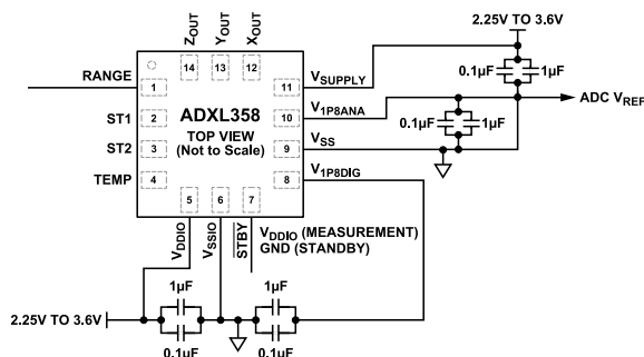
Figure 26. ADXL358 Application Circuit
