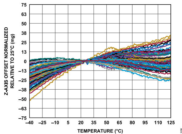
Figure 8. Zero g Offset Normalized Relative to 25°C vs. Temperature, Z-Axis
