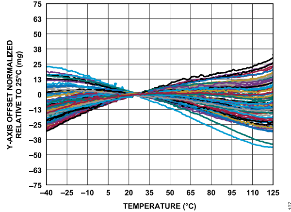
Figure 7. Zero g Offset Normalized Relative to 25°C vs. Temperature, Y-Axis
