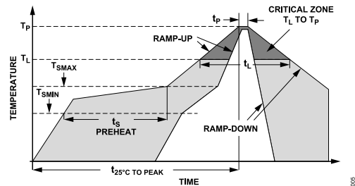
Figure 28. Recommended Soldering Profile
