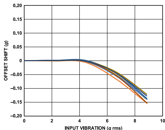
Figure 18. VRE, X-Axis Offset from +1 g, \pm 10 g Range, X-Axis Orientation = +1 g
