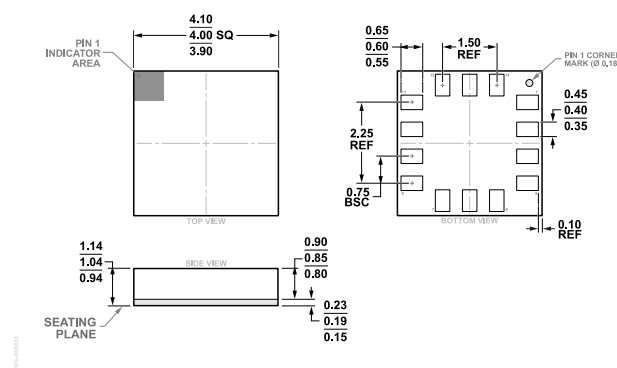
Figure 30. 14-Terminal Land Grid Array [LGA] (CC-14-2) Dimensions shown in millimeters
