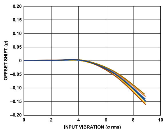
Figure 19. VRE, Y-Axis Offset from +1 g, \pm 10 g Range, Y-Axis Orientation = +1 g
