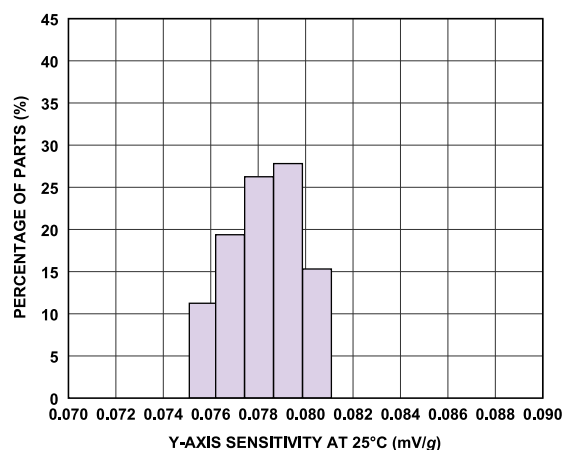
Figure 16. Sensitivity Histogram at 25°C, Y-Axis
