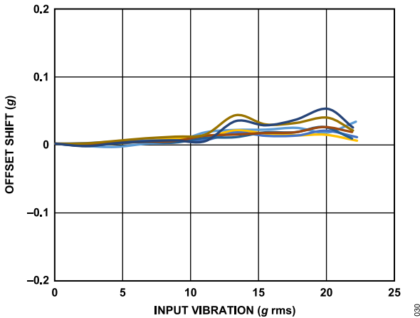
Figure 22. VRE, Y-Axis Offset from -1 g, \pm 40 g Range, Y-Axis Orientation = -1 g
