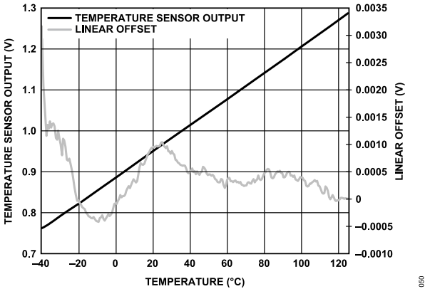
Figure 24. Temperature Sensor Output and Linear Offset vs. Temperature
