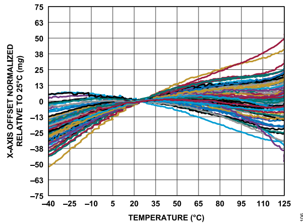
Figure 6. Zero g Offset Normalized Relative to 25°C vs. Temperature, X-Axis
