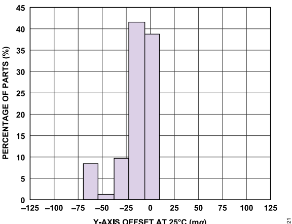
Figure 13. Zero g Offset Histogram at 25°C, Y-Axis
