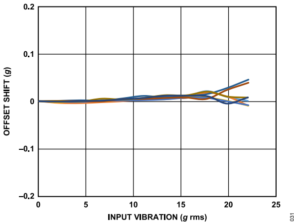
Figure 23. VRE, Z-Axis Offset from -1 g, \pm 40 g Range, Z-Axis Orientation = -1 g
