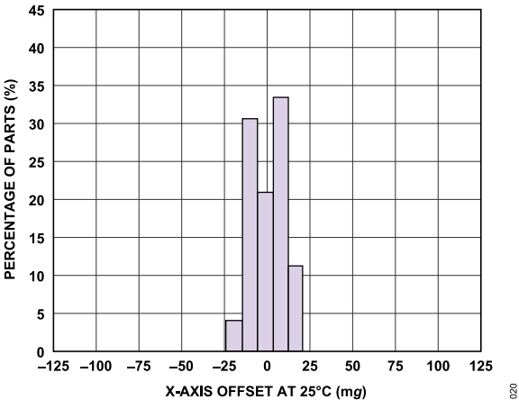
Figure 12. Zero g Offset Histogram at 25°C, X-Axis
