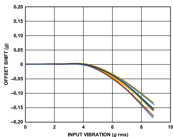
Figure 20. VRE, Z-Axis Offset from +1 g, \pm 10 g Range, Z-Axis Orientation = +1 g
