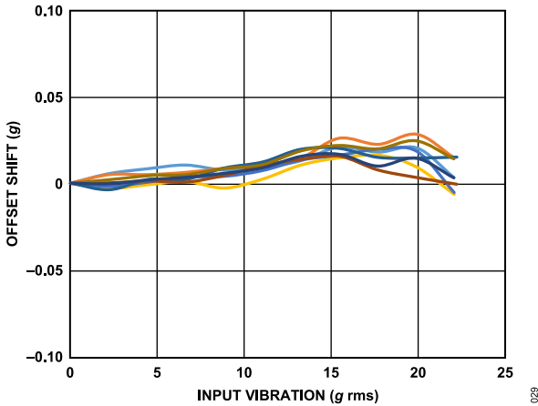
Figure 21. VRE, X-Axis Offset from -1 g, \pm 40 g Range, X-Axis Orientation = -1 g
