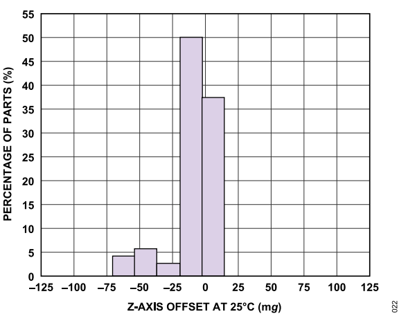
Figure 14. Zero g Offset Histogram at 25°C, Z-Axis
